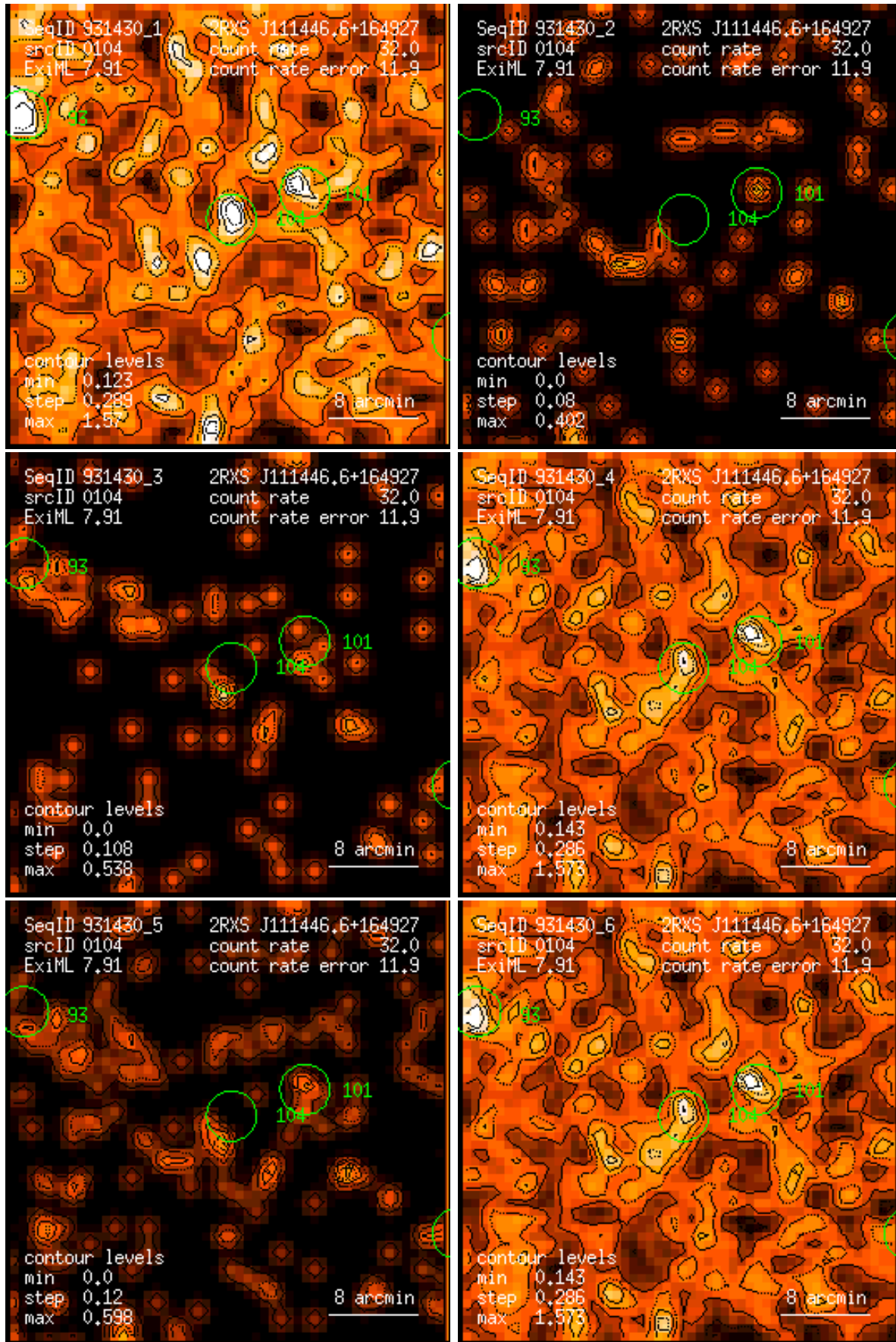
Figure 104: RASS 931430: detection 0104: band rate images, Gaussian filter: (1) PSPC channels 11 – 41, (2) 52 – 90, (3) 91 – 201, (4) 11 – 235, (5) 52 – 201, (6) 11 – 201. Broad band rates in counts/ks. Band rate contour levels in counts/ks/arcmin 2 .
