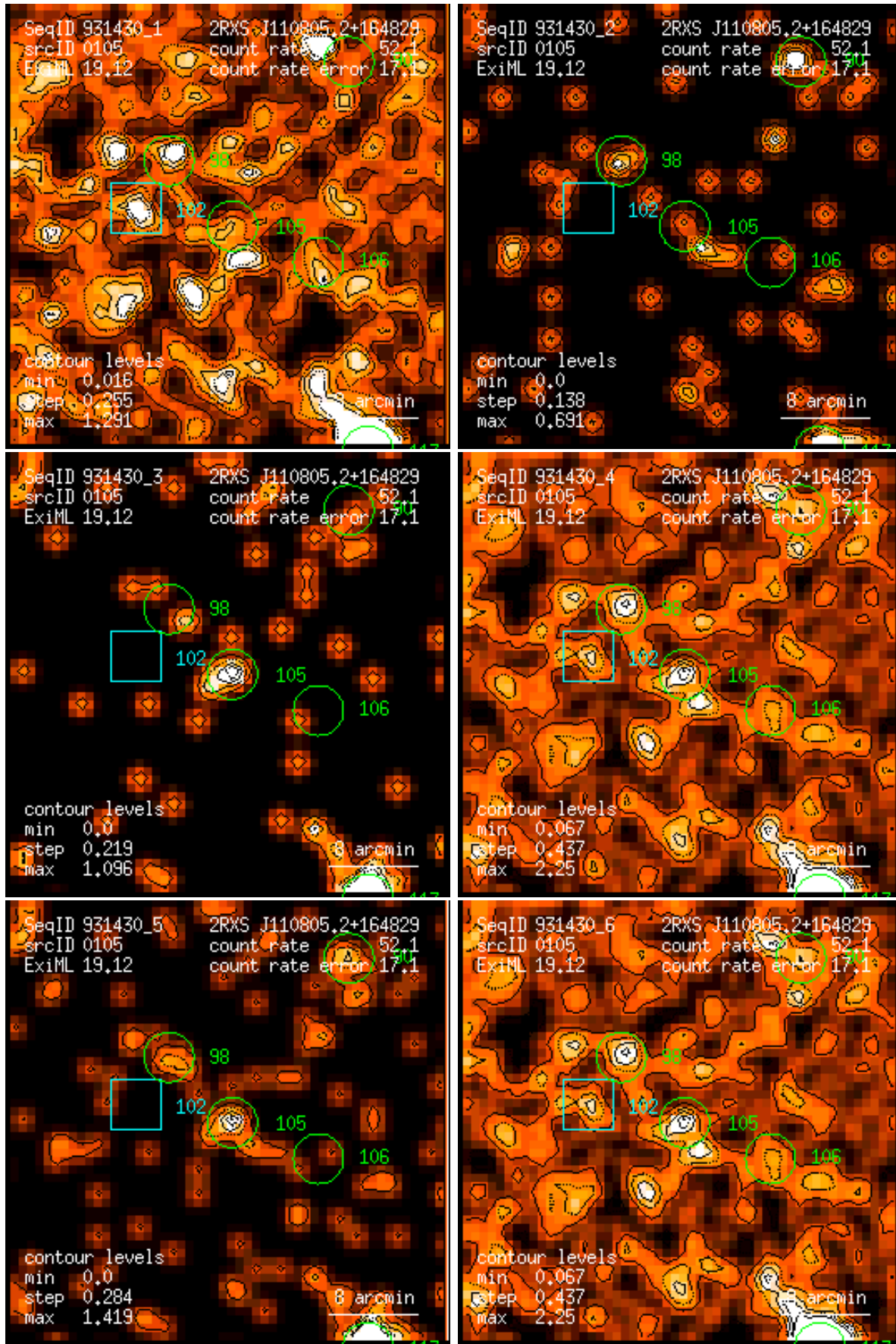
Figure 105: RASS 931430: detection 0105: band rate images, Gaussian filter: (1) PSPC channels 11 – 41, (2) 52 – 90, (3) 91 – 201, (4) 11 – 235, (5) 52 – 201, (6) 11 – 201. Broad band rates in counts/ks. Band rate contour levels in counts/ks/arcmin 2 .
