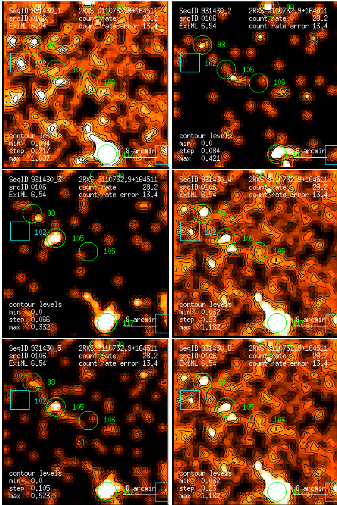
Figure 106: RASS 931430: detection 0106: band rate images, Gaussian filter: (1) PSPC channels 11 – 41, (2) 52 – 90, (3) 91 – 201, (4) 11 – 235, (5) 52 – 201, (6) 11 – 201. Broad band rates in counts/ks. Band rate contour levels in counts/ks/arcmin 2 .
