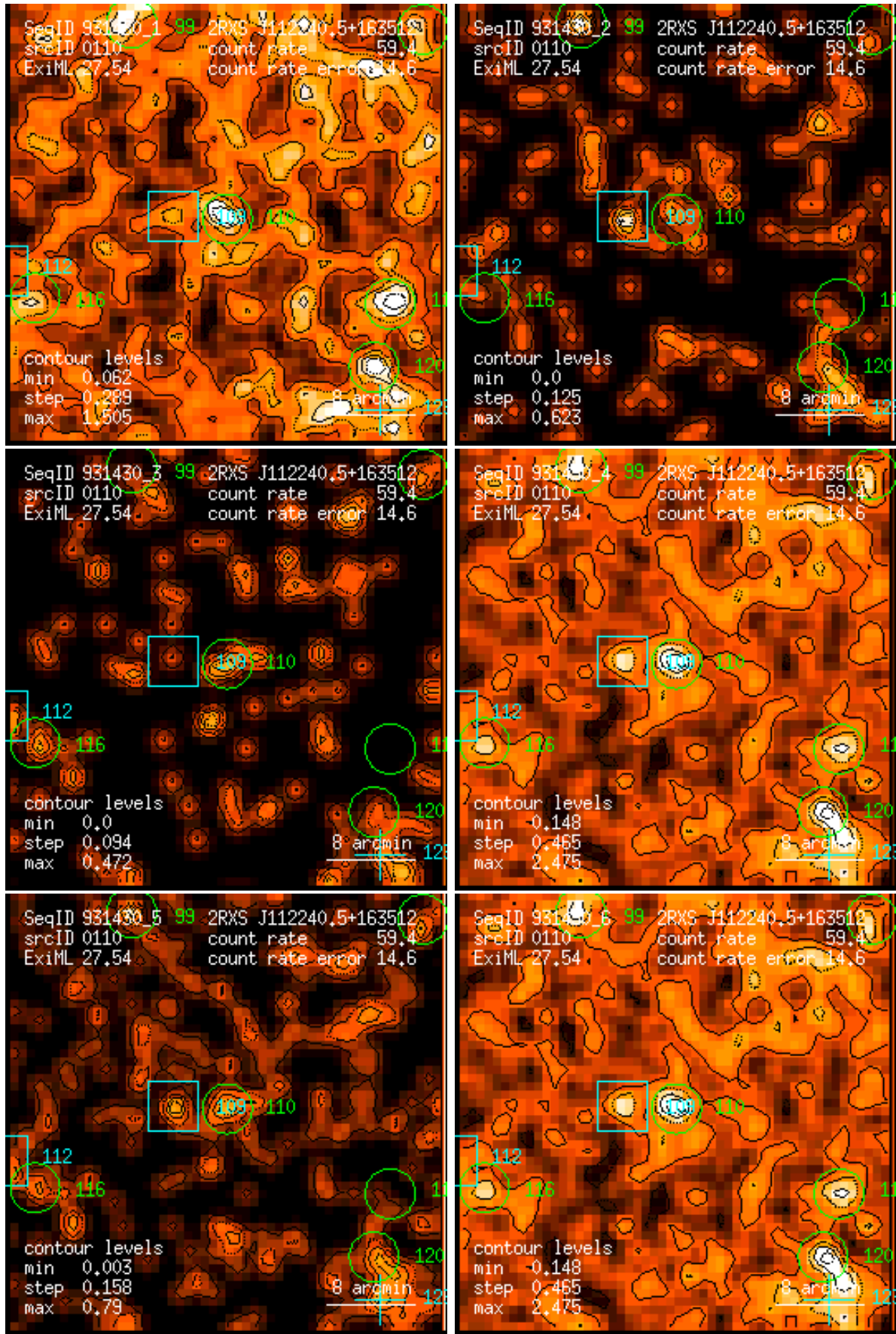
Figure 110: RASS 931430: detection 0110: band rate images, Gaussian filter: (1) PSPC channels 11 – 41, (2) 52 – 90, (3) 91 – 201, (4) 11 – 235, (5) 52 – 201, (6) 11 – 201. Broad band rates in counts/ks. Band rate contour levels in counts/ks/arcmin 2 .
