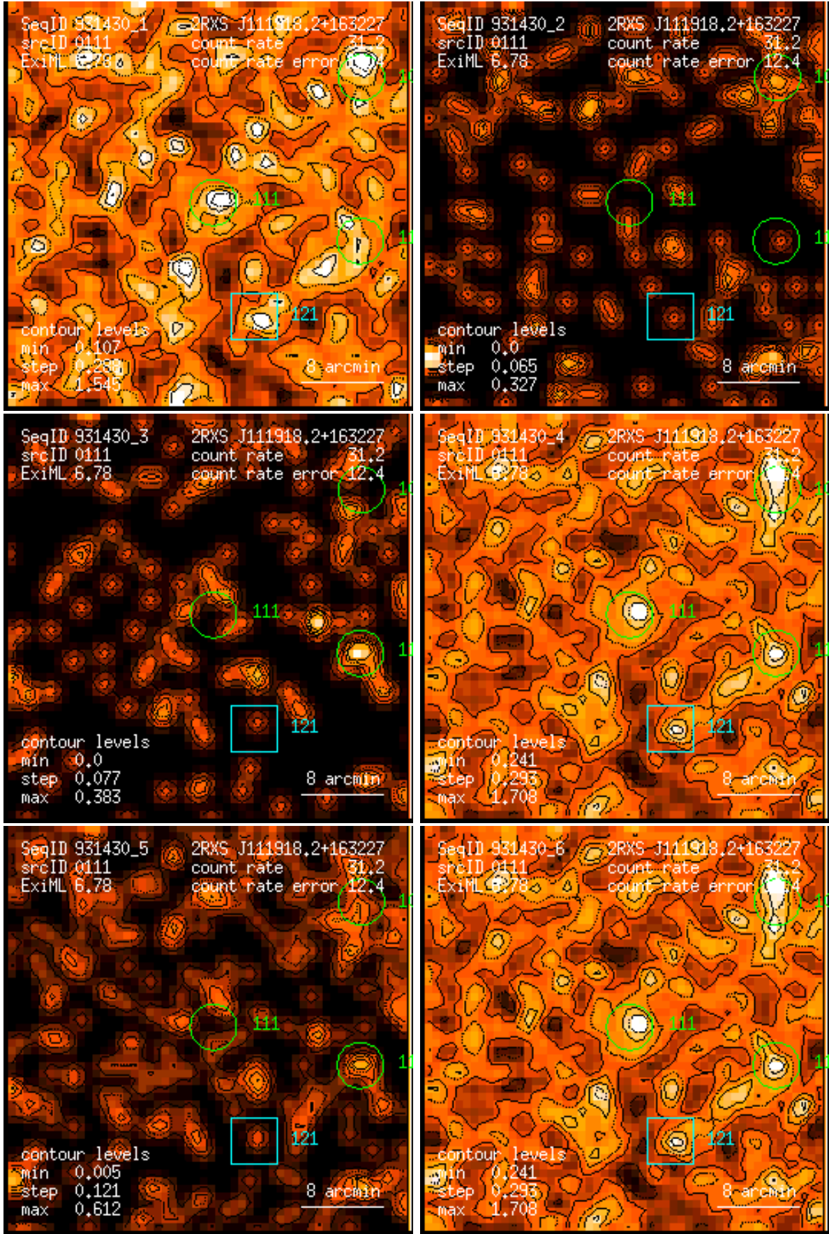
Figure 111: RASS 931430: detection 0111: band rate images, Gaussian filter: (1) PSPC channels 11 – 41, (2) 52 – 90, (3) 91 – 201, (4) 11 – 235, (5) 52 – 201, (6) 11 – 201. Broad band rates in counts/ks. Band rate contour levels in counts/ks/arcmin 2 .
