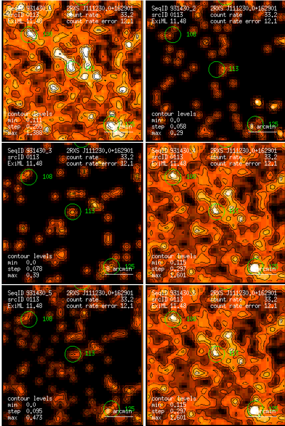
Figure 113: RASS 931430: detection 0113: band rate images, Gaussian filter: (1) PSPC channels 11 – 41, (2) 52 – 90, (3) 91 – 201, (4) 11 – 235, (5) 52 – 201, (6) 11 – 201. Broad band rates in counts/ks. Band rate contour levels in counts/ks/arcmin 2 .
