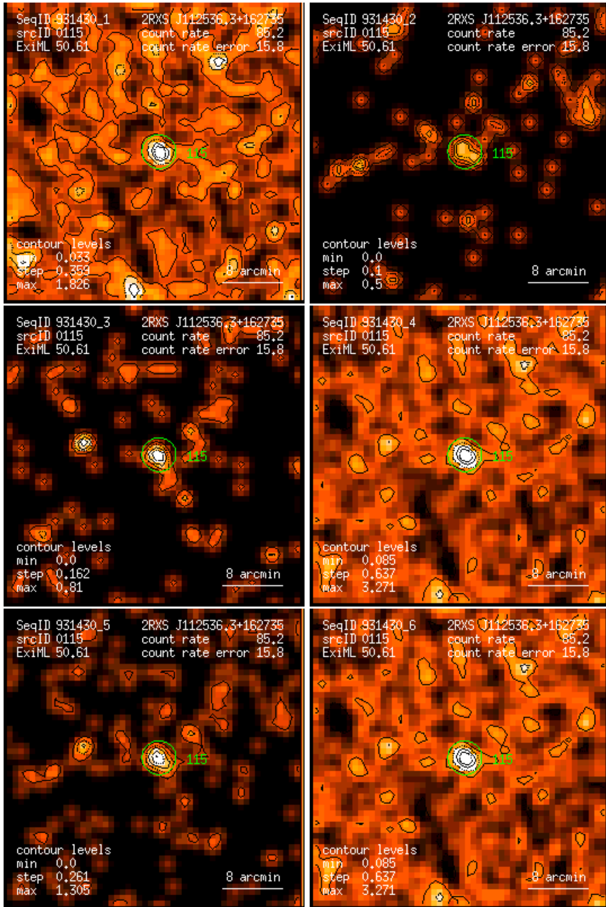
Figure 115: RASS 931430: detection 0115: band rate images, Gaussian filter: (1) PSPC channels 11 – 41, (2) 52 – 90, (3) 91 – 201, (4) 11 – 235, (5) 52 – 201, (6) 11 – 201. Broad band rates in counts/ks. Band rate contour levels in counts/ks/arcmin 2 .
