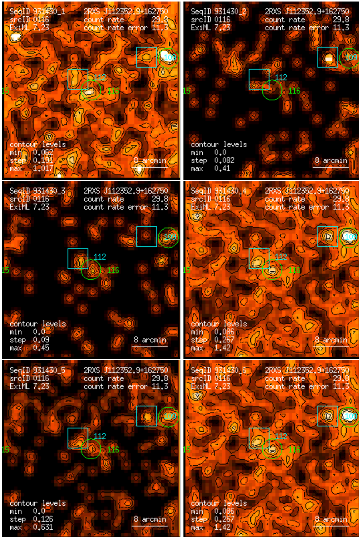
Figure 116: RASS 931430: detection 0116: band rate images, Gaussian filter: (1) PSPC channels 11 – 41, (2) 52 – 90, (3) 91 – 201, (4) 11 – 235, (5) 52 – 201, (6) 11 – 201. Broad band rates in counts/ks. Band rate contour levels in counts/ks/arcmin 2 .
