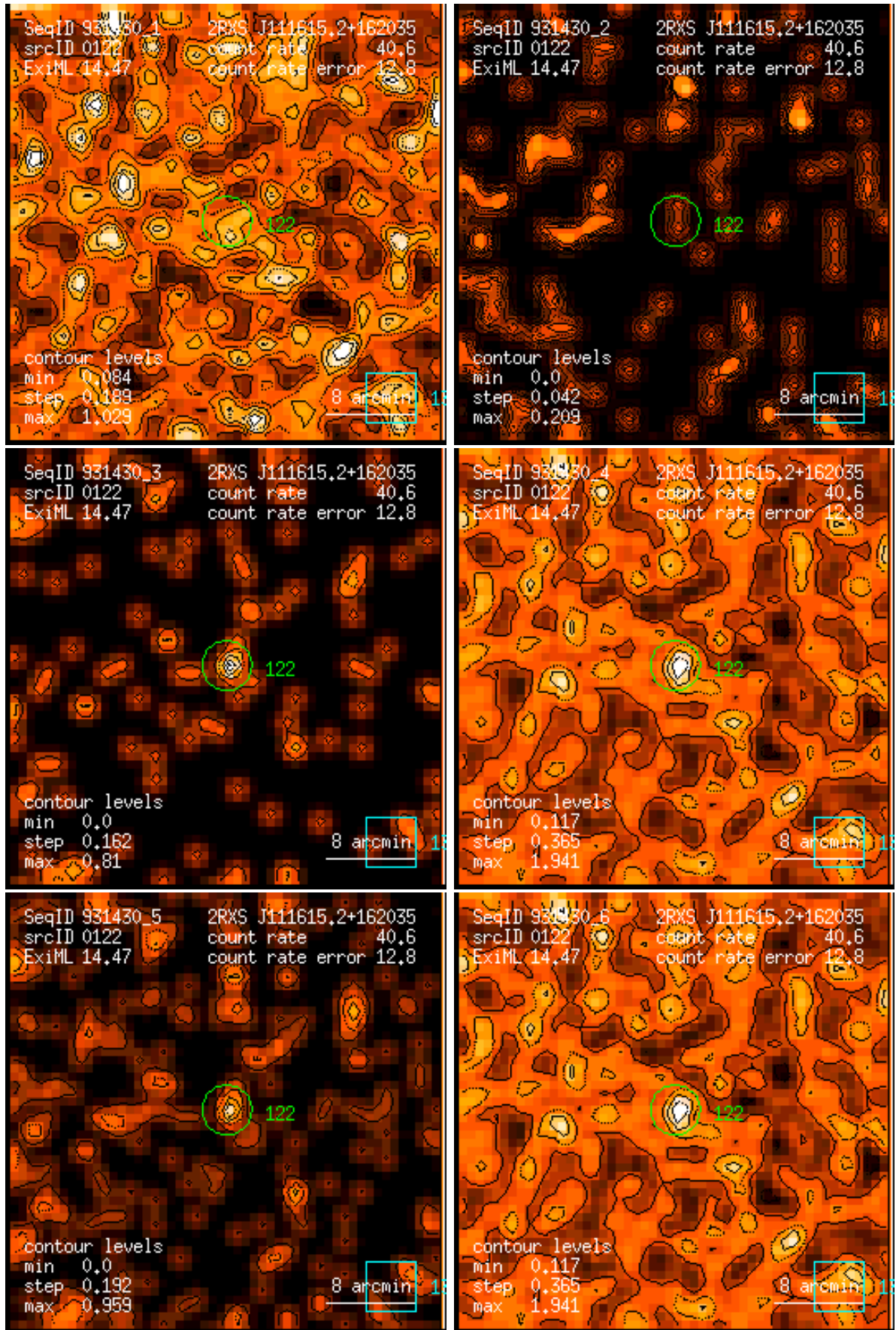
Figure 122: RASS 931430: detection 0122: band rate images, Gaussian filter: (1) PSPC channels 11 – 41, (2) 52 – 90, (3) 91 – 201, (4) 11 – 235, (5) 52 – 201, (6) 11 – 201. Broad band rates in counts/ks. Band rate contour levels in counts/ks/arcmin 2 .
