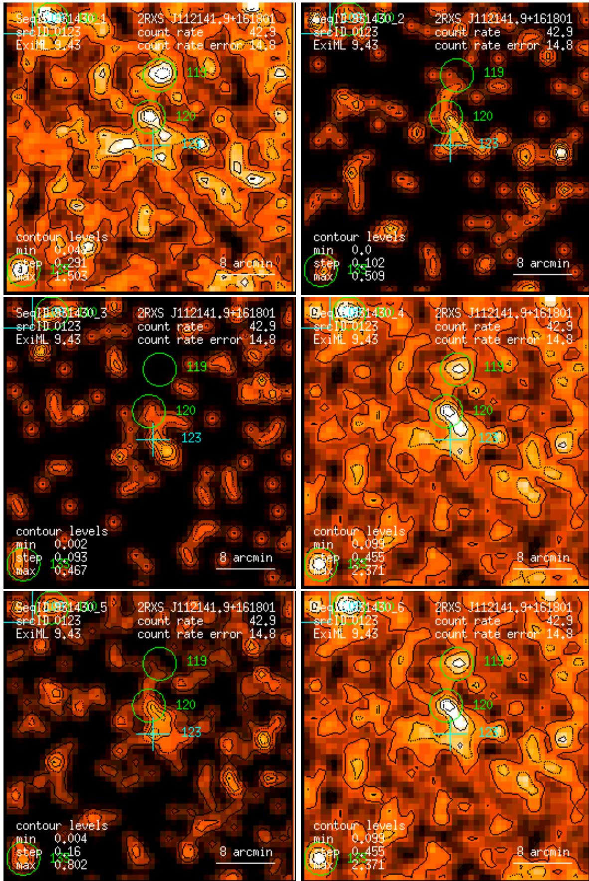
Figure 123: RASS 931430: detection 0123: band rate images, Gaussian filter: (1) PSPC channels 11 – 41, (2) 52 – 90, (3) 91 – 201, (4) 11 – 235, (5) 52 – 201, (6) 11 – 201. Broad band rates in counts/ks. Band rate contour levels in counts/ks/arcmin 2 .
