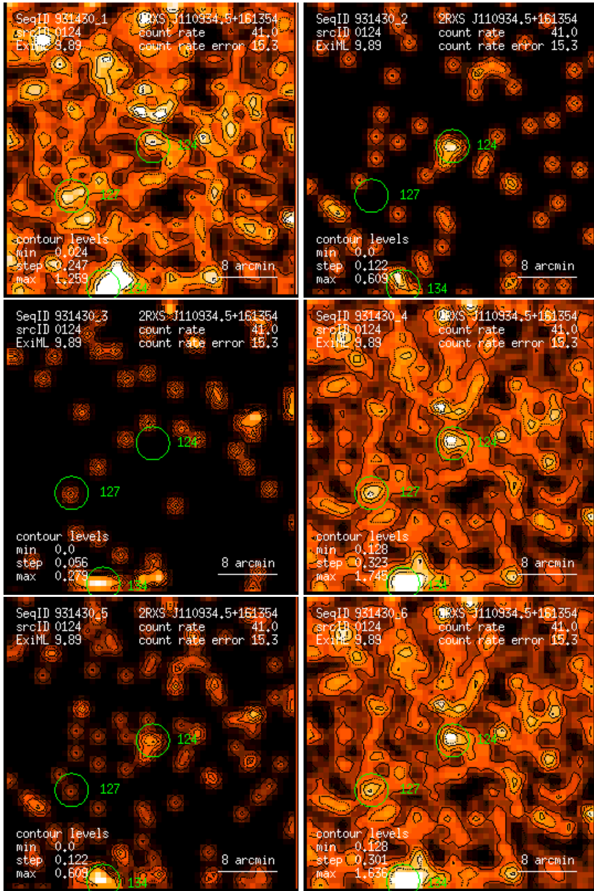
Figure 124: RASS 931430: detection 0124: band rate images, Gaussian filter: (1) PSPC channels 11 – 41, (2) 52 – 90, (3) 91 – 201, (4) 11 – 235, (5) 52 – 201, (6) 11 – 201. Broad band rates in counts/ks. Band rate contour levels in counts/ks/arcmin 2 .
