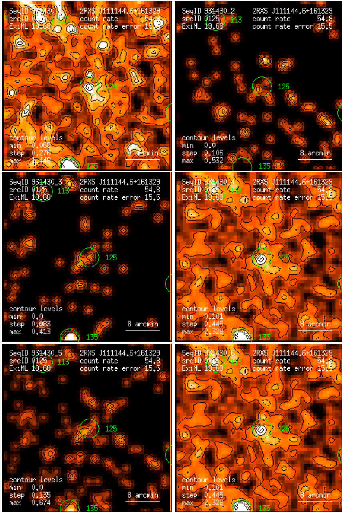
Figure 125: RASS 931430: detection 0125: band rate images, Gaussian filter: (1) PSPC channels 11 – 41, (2) 52 – 90, (3) 91 – 201, (4) 11 – 235, (5) 52 – 201, (6) 11 – 201. Broad band rates in counts/ks. Band rate contour levels in counts/ks/arcmin 2 .
