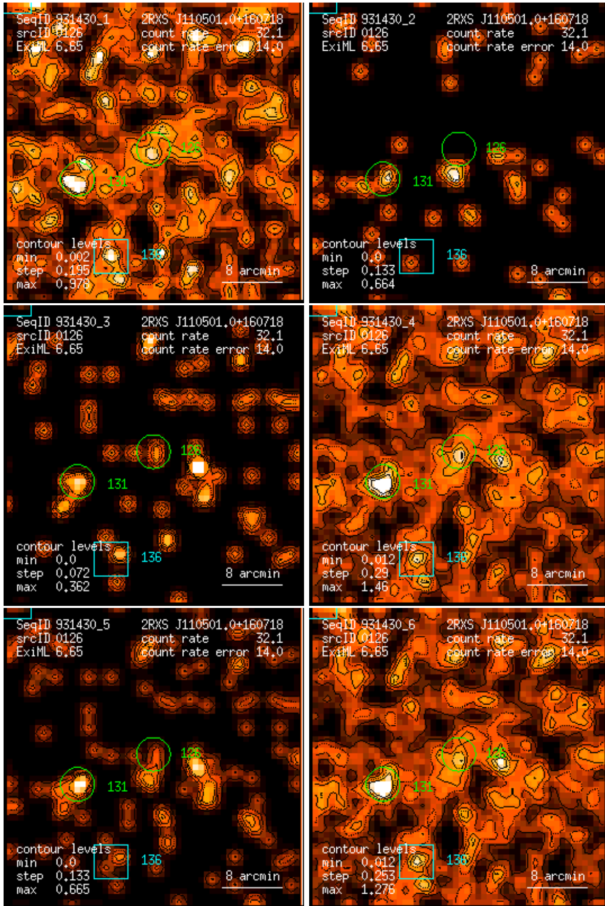
Figure 126: RASS 931430: detection 0126: band rate images, Gaussian filter: (1) PSPC channels 11 – 41, (2) 52 – 90, (3) 91 – 201, (4) 11 – 235, (5) 52 – 201, (6) 11 – 201. Broad band rates in counts/ks. Band rate contour levels in counts/ks/arcmin 2 .
