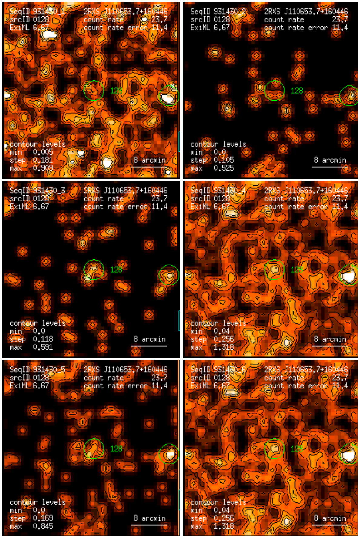
Figure 128: RASS 931430: detection 0128: band rate images, Gaussian filter: (1) PSPC channels 11 – 41, (2) 52 – 90, (3) 91 – 201, (4) 11 – 235, (5) 52 – 201, (6) 11 – 201. Broad band rates in counts/ks. Band rate contour levels in counts/ks/arcmin 2 .
