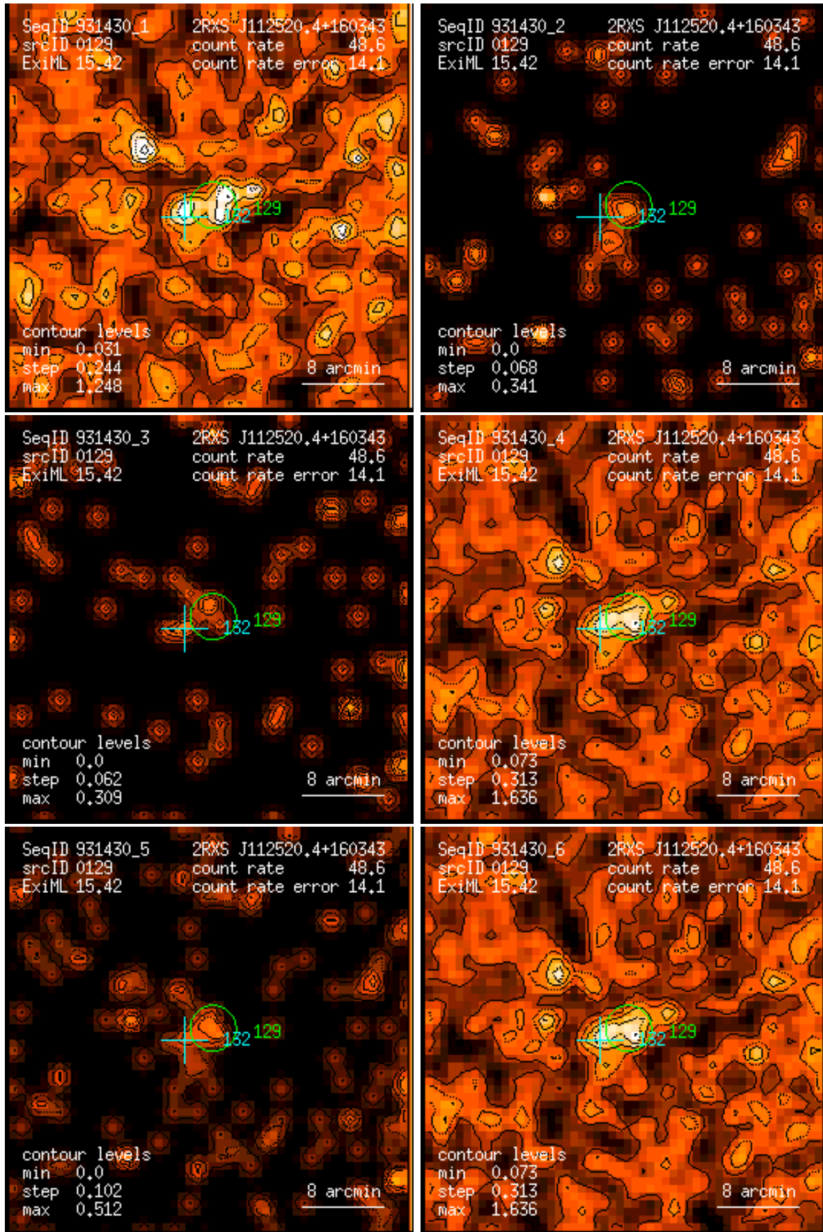
Figure 129: RASS 931430: detection 0129: band rate images, Gaussian filter: (1) PSPC channels 11 – 41, (2) 52 – 90, (3) 91 – 201, (4) 11 – 235, (5) 52 – 201, (6) 11 – 201. Broad band rates in counts/ks. Band rate contour levels in counts/ks/arcmin 2 .
