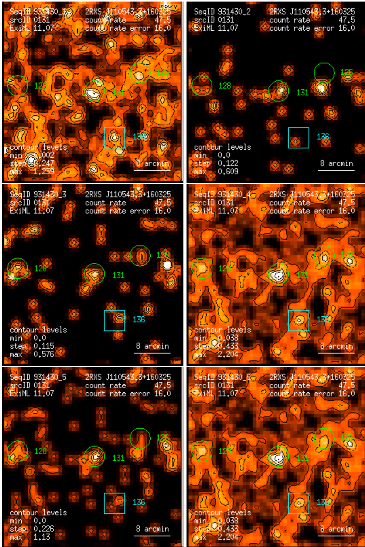
Figure 131: RASS 931430: detection 0131: band rate images, Gaussian filter: (1) PSPC channels 11 – 41, (2) 52 – 90, (3) 91 – 201, (4) 11 – 235, (5) 52 – 201, (6) 11 – 201. Broad band rates in counts/ks. Band rate contour levels in counts/ks/arcmin 2 .
