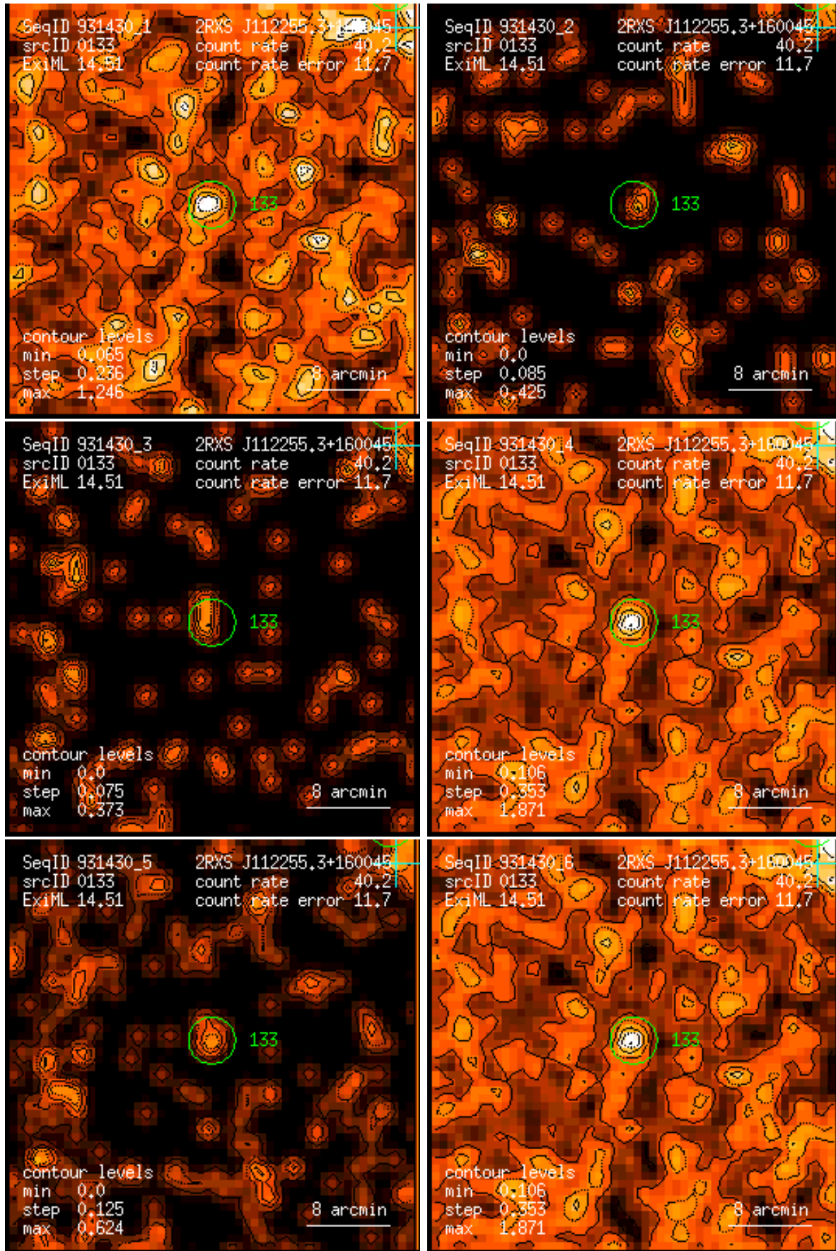
Figure 133: RASS 931430: detection 0133: band rate images, Gaussian filter: (1) PSPC channels 11 – 41, (2) 52 – 90, (3) 91 – 201, (4) 11 – 235, (5) 52 – 201, (6) 11 – 201. Broad band rates in counts/ks. Band rate contour levels in counts/ks/arcmin 2 .
