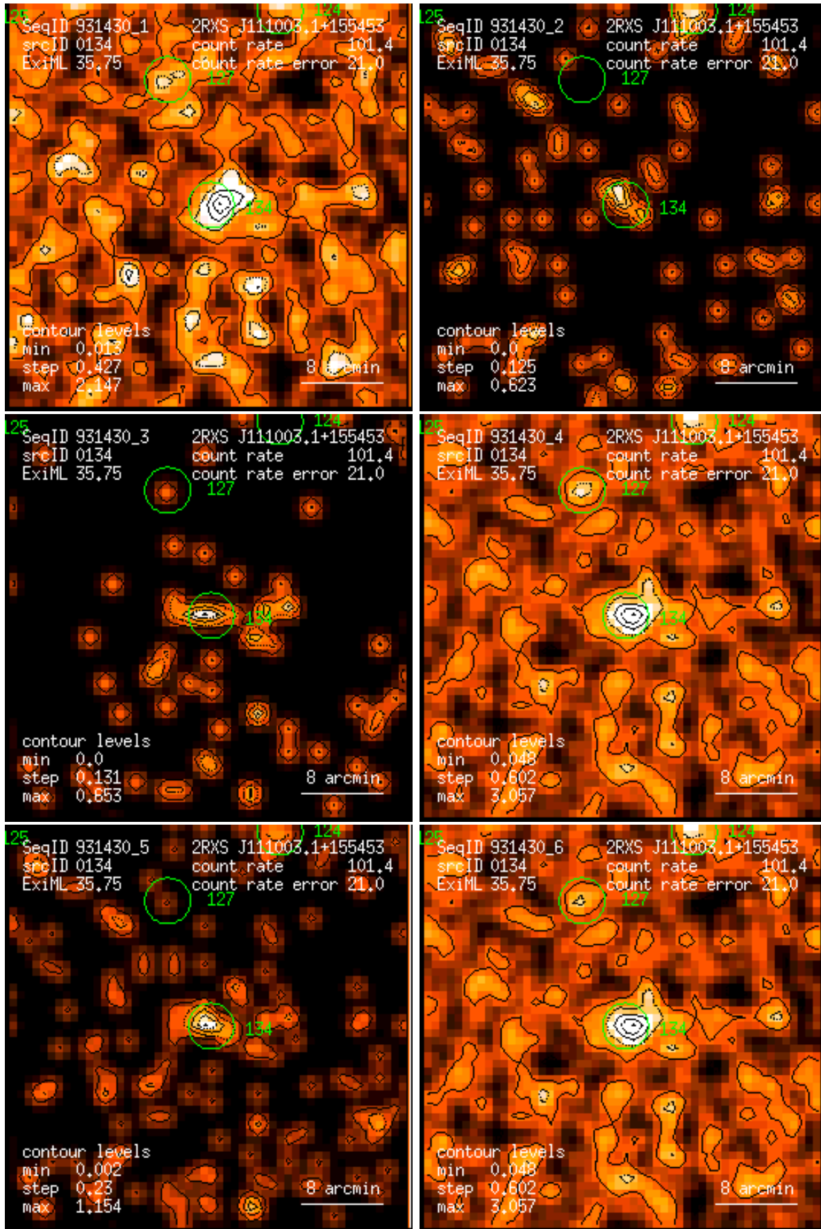
Figure 134: RASS 931430: detection 0134: band rate images, Gaussian filter: (1) PSPC channels 11 – 41, (2) 52 – 90, (3) 91 – 201, (4) 11 – 235, (5) 52 – 201, (6) 11 – 201. Broad band rates in counts/ks. Band rate contour levels in counts/ks/arcmin 2 .
