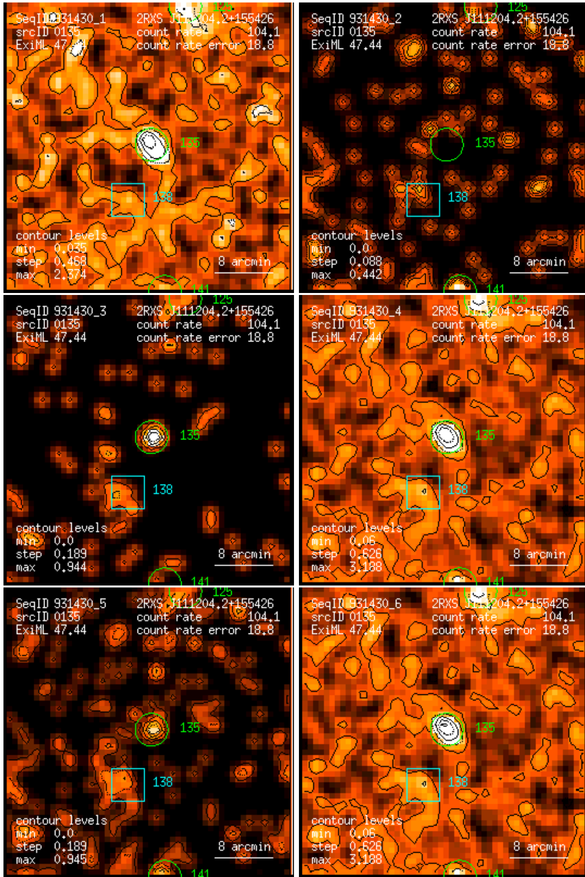
Figure 135: RASS 931430: detection 0135: band rate images, Gaussian filter: (1) PSPC channels 11 – 41, (2) 52 – 90, (3) 91 – 201, (4) 11 – 235, (5) 52 – 201, (6) 11 – 201. Broad band rates in counts/ks. Band rate contour levels in counts/ks/arcmin 2 .
