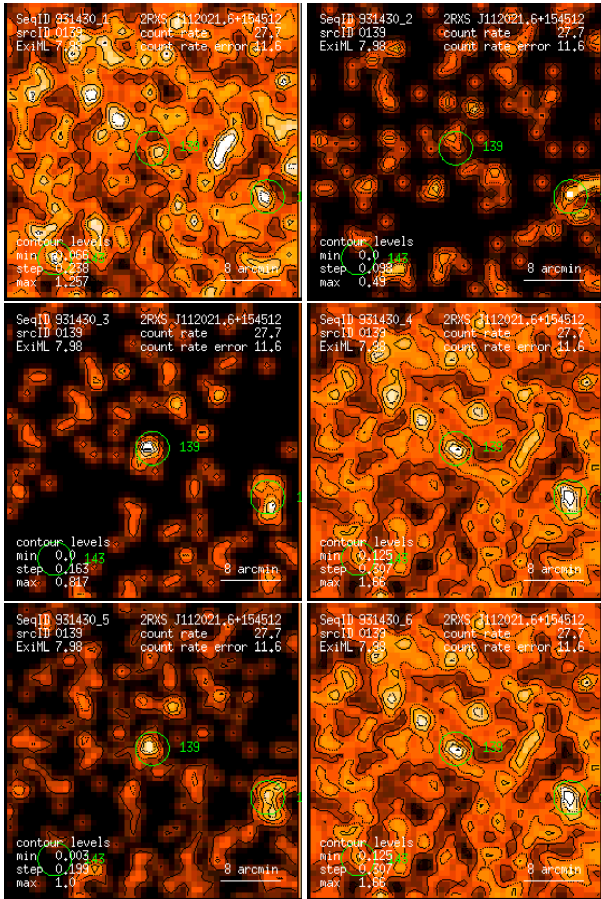
Figure 139: RASS 931430: detection 0139: band rate images, Gaussian filter: (1) PSPC channels 11 – 41, (2) 52 – 90, (3) 91 – 201, (4) 11 – 235, (5) 52 – 201, (6) 11 – 201. Broad band rates in counts/ks. Band rate contour levels in counts/ks/arcmin 2 .
