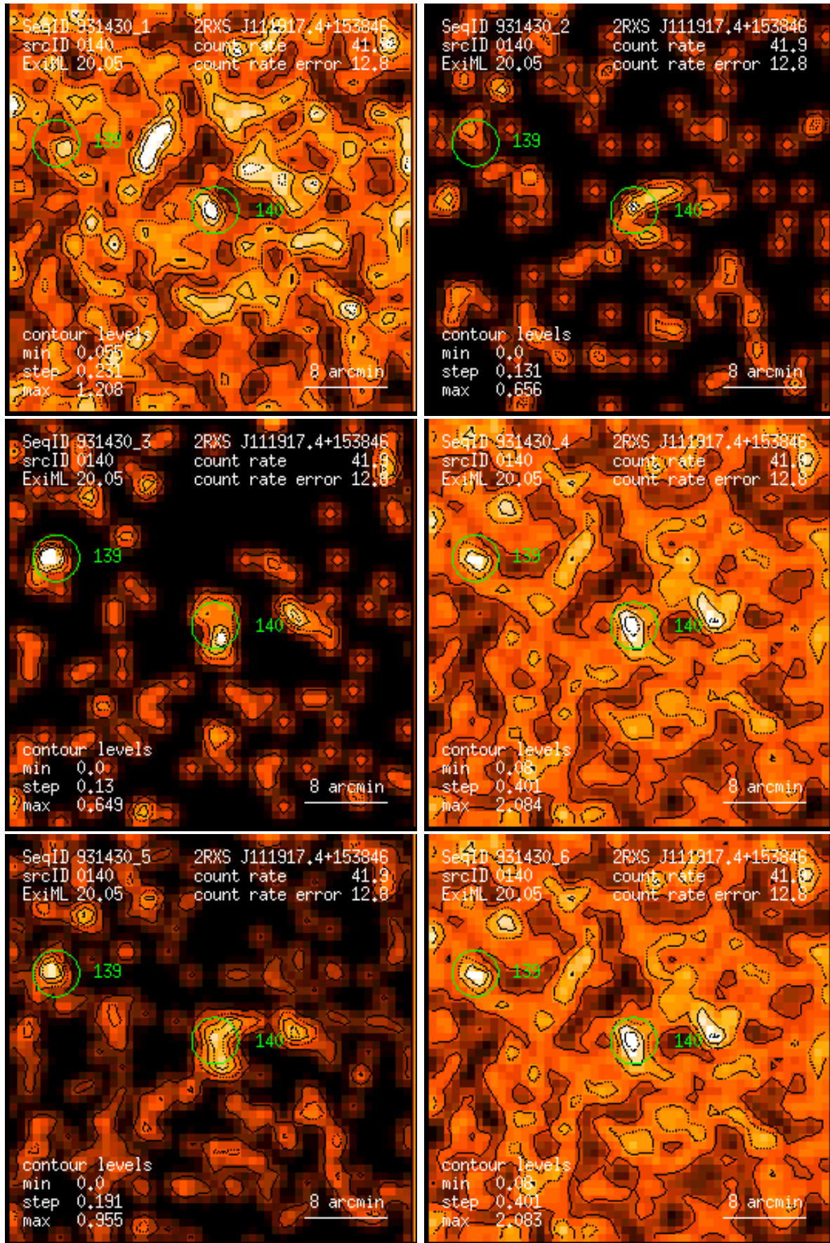
Figure 140: RASS 931430: detection 0140: band rate images, Gaussian filter: (1) PSPC channels 11 – 41, (2) 52 – 90, (3) 91 – 201, (4) 11 – 235, (5) 52 – 201, (6) 11 – 201. Broad band rates in counts/ks. Band rate contour levels in counts/ks/arcmin 2 .
