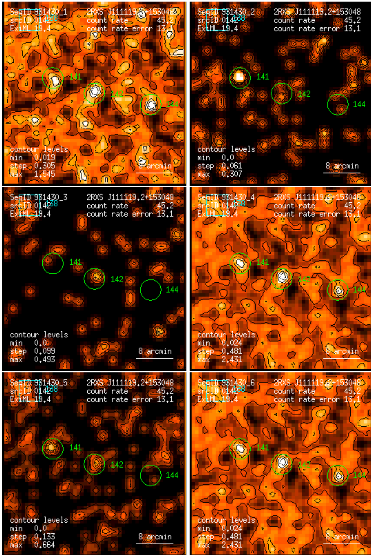
Figure 142: RASS 931430: detection 0142: band rate images, Gaussian filter: (1) PSPC channels 11 – 41, (2) 52 – 90, (3) 91 – 201, (4) 11 – 235, (5) 52 – 201, (6) 11 – 201. Broad band rates in counts/ks. Band rate contour levels in counts/ks/arcmin 2 .
