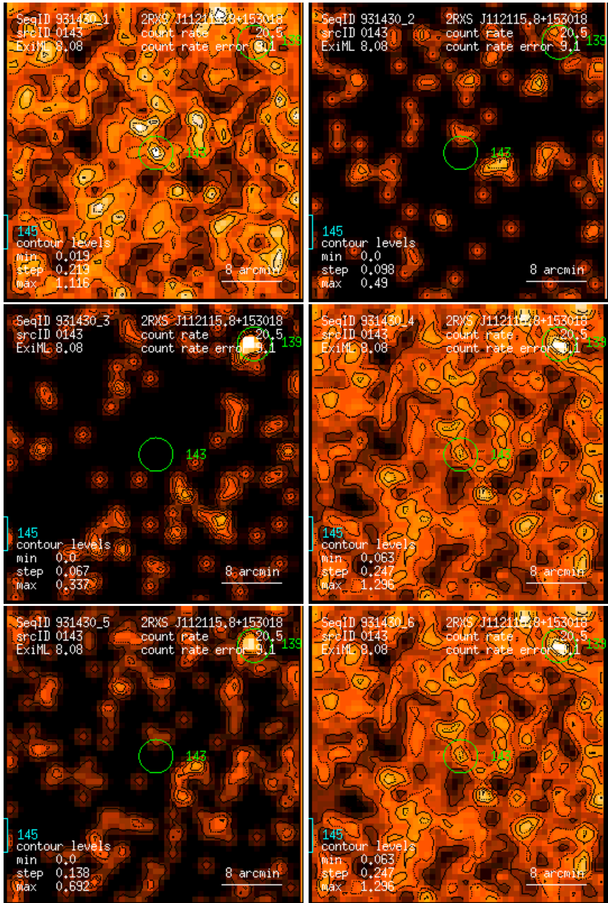
Figure 143: RASS 931430: detection 0143: band rate images, Gaussian filter: (1) PSPC channels 11 – 41, (2) 52 – 90, (3) 91 – 201, (4) 11 – 235, (5) 52 – 201, (6) 11 – 201. Broad band rates in counts/ks. Band rate contour levels in counts/ks/arcmin 2 .
