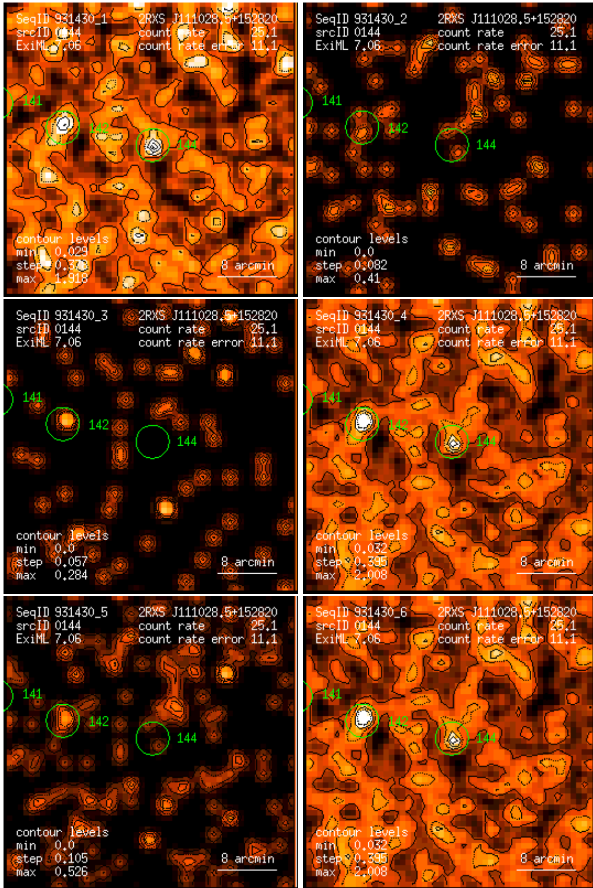
Figure 144: RASS 931430: detection 0144: band rate images, Gaussian filter: (1) PSPC channels 11 – 41, (2) 52 – 90, (3) 91 – 201, (4) 11 – 235, (5) 52 – 201, (6) 11 – 201. Broad band rates in counts/ks. Band rate contour levels in counts/ks/arcmin 2 .
