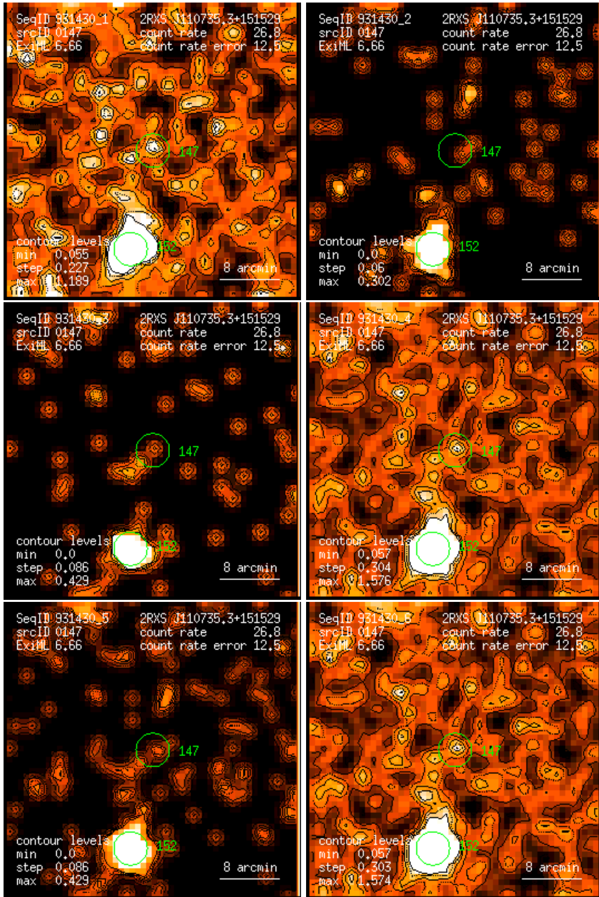
Figure 147: RASS 931430: detection 0147: band rate images, Gaussian filter: (1) PSPC channels 11 – 41, (2) 52 – 90, (3) 91 – 201, (4) 11 – 235, (5) 52 – 201, (6) 11 – 201. Broad band rates in counts/ks. Band rate contour levels in counts/ks/arcmin 2 .
