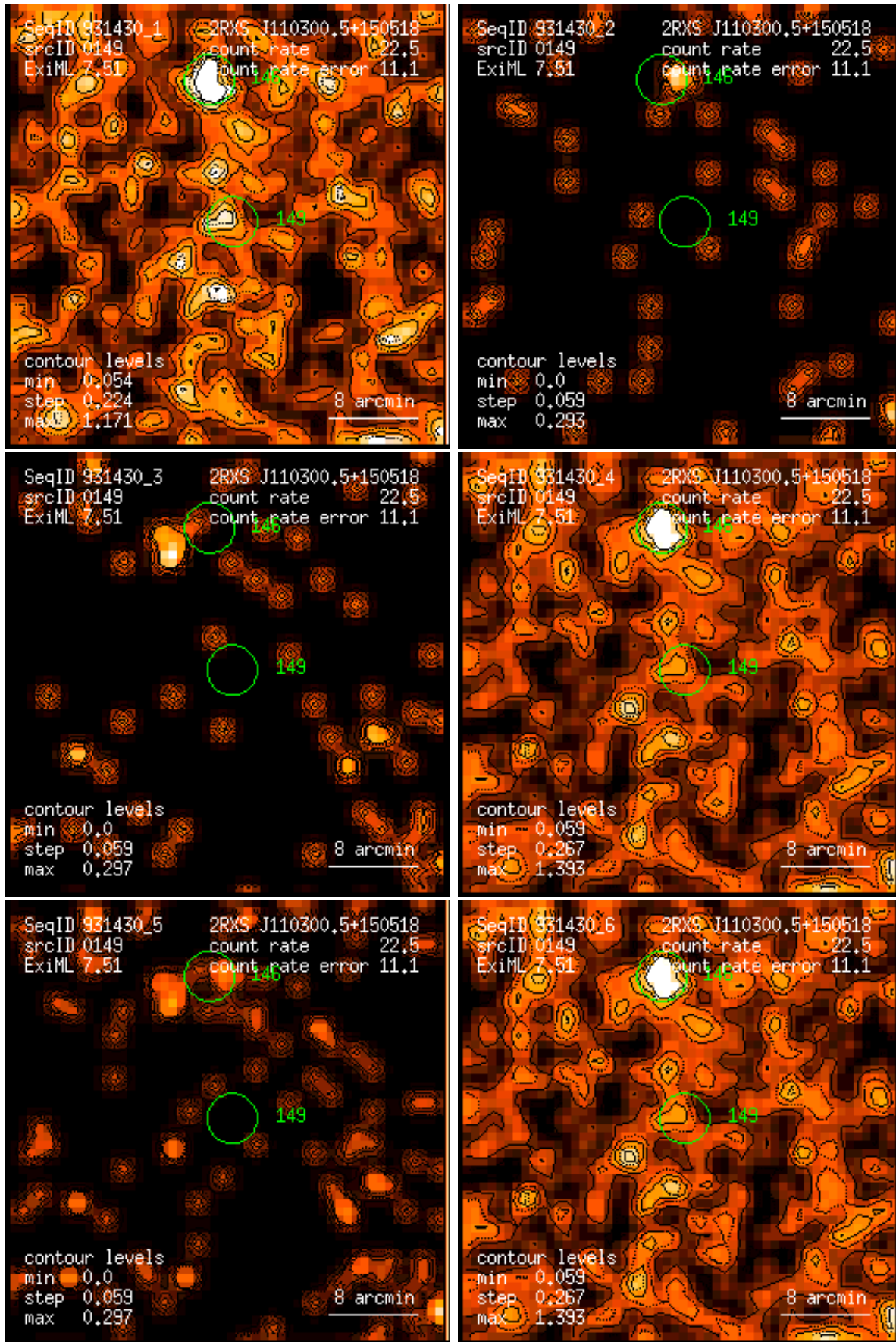
Figure 149: RASS 931430: detection 0149: band rate images, Gaussian filter: (1) PSPC channels 11 – 41, (2) 52 – 90, (3) 91 – 201, (4) 11 – 235, (5) 52 – 201, (6) 11 – 201. Broad band rates in counts/ks. Band rate contour levels in counts/ks/arcmin 2 .
