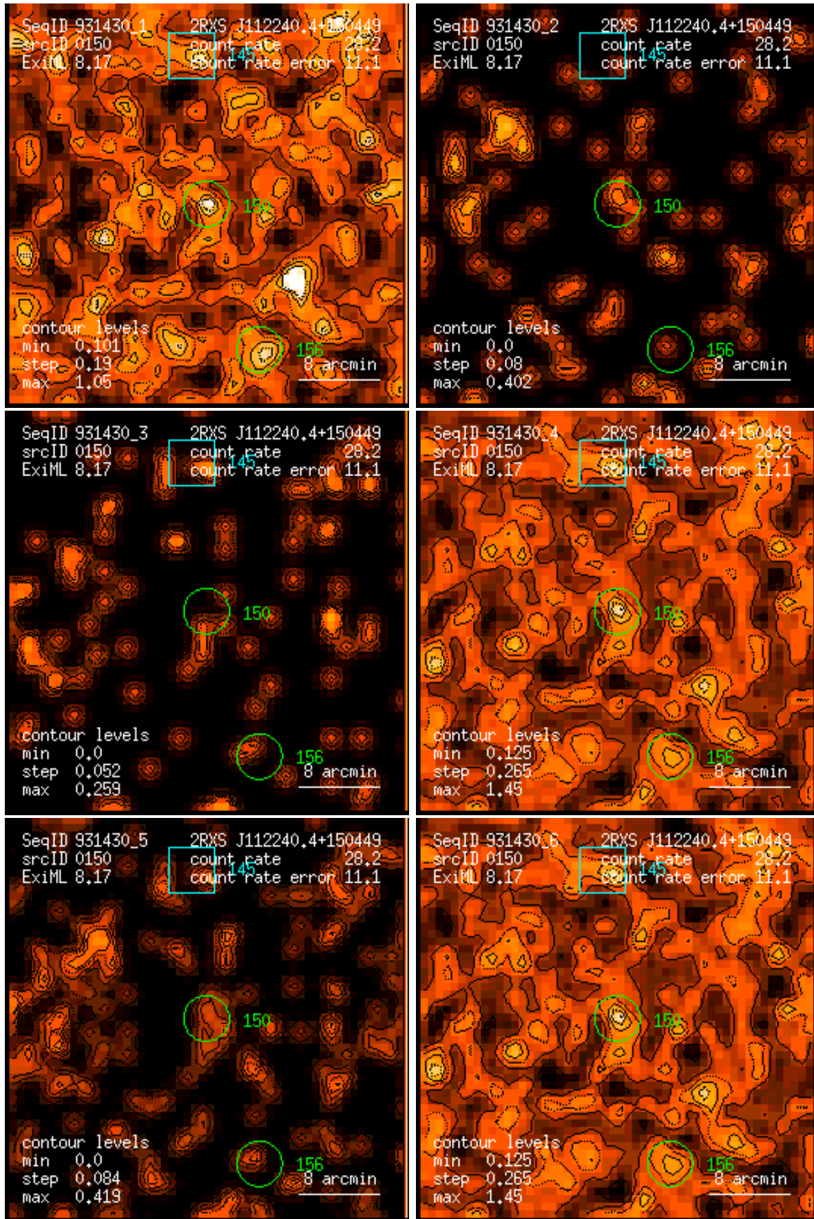
Figure 150: RASS 931430: detection 0150: band rate images, Gaussian filter: (1) PSPC channels 11 – 41, (2) 52 – 90, (3) 91 – 201, (4) 11 – 235, (5) 52 – 201, (6) 11 – 201. Broad band rates in counts/ks. Band rate contour levels in counts/ks/arcmin 2 .
