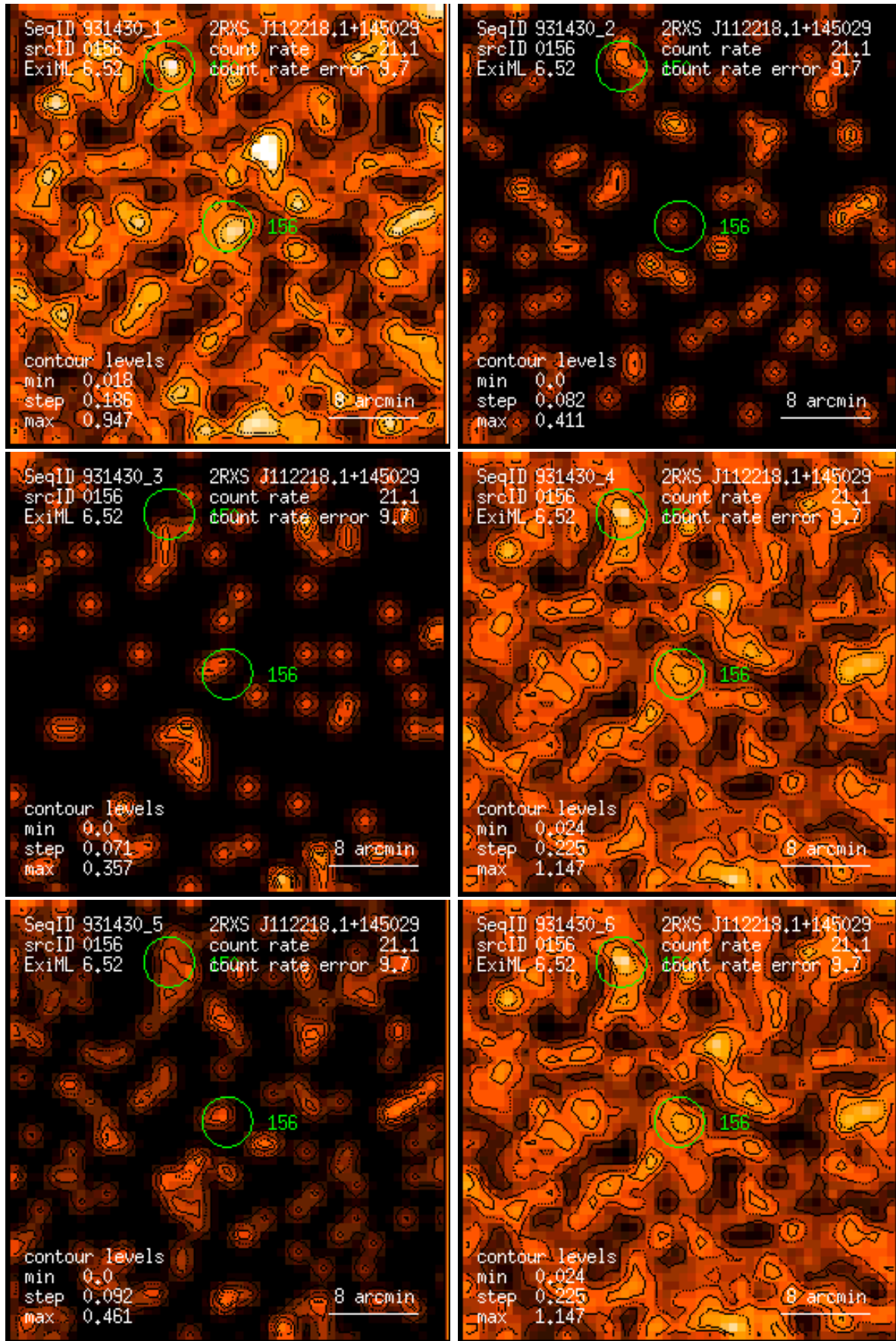
Figure 156: RASS 931430: detection 0156: band rate images, Gaussian filter: (1) PSPC channels 11 – 41, (2) 52 – 90, (3) 91 – 201, (4) 11 – 235, (5) 52 – 201, (6) 11 – 201. Broad band rates in counts/ks. Band rate contour levels in counts/ks/arcmin 2 .
