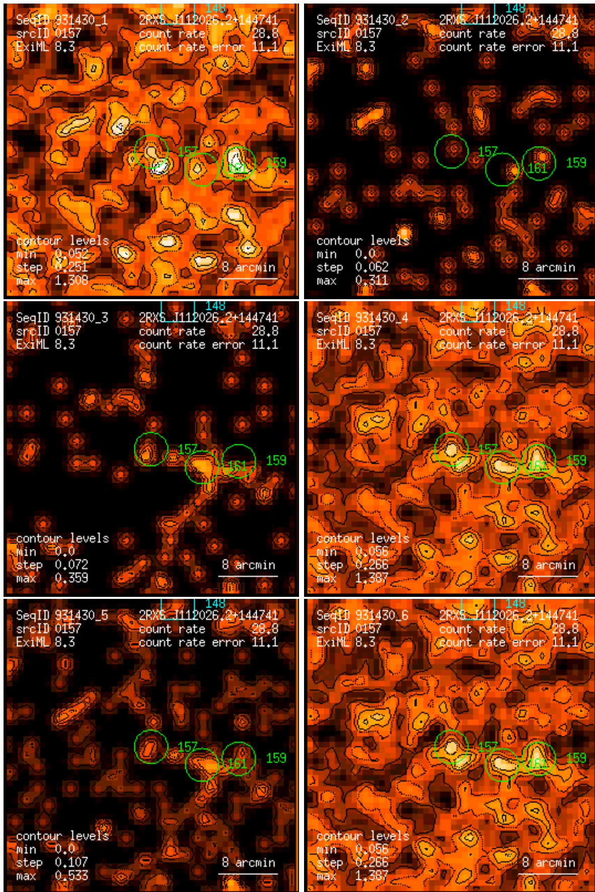
Figure 157: RASS 931430: detection 0157: band rate images, Gaussian filter: (1) PSPC channels 11 – 41, (2) 52 – 90, (3) 91 – 201, (4) 11 – 235, (5) 52 – 201, (6) 11 – 201. Broad band rates in counts/ks. Band rate contour levels in counts/ks/arcmin 2 .
