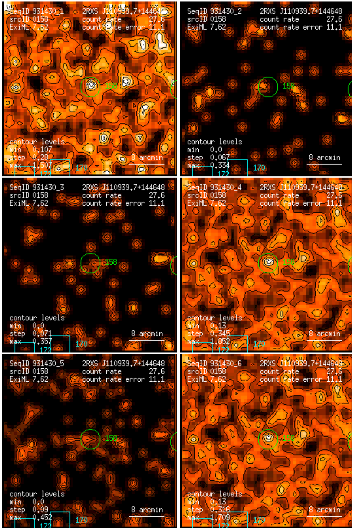
Figure 158: RASS 931430: detection 0158: band rate images, Gaussian filter: (1) PSPC channels 11 – 41, (2) 52 – 90, (3) 91 – 201, (4) 11 – 235, (5) 52 – 201, (6) 11 – 201. Broad band rates in counts/ks. Band rate contour levels in counts/ks/arcmin 2 .
