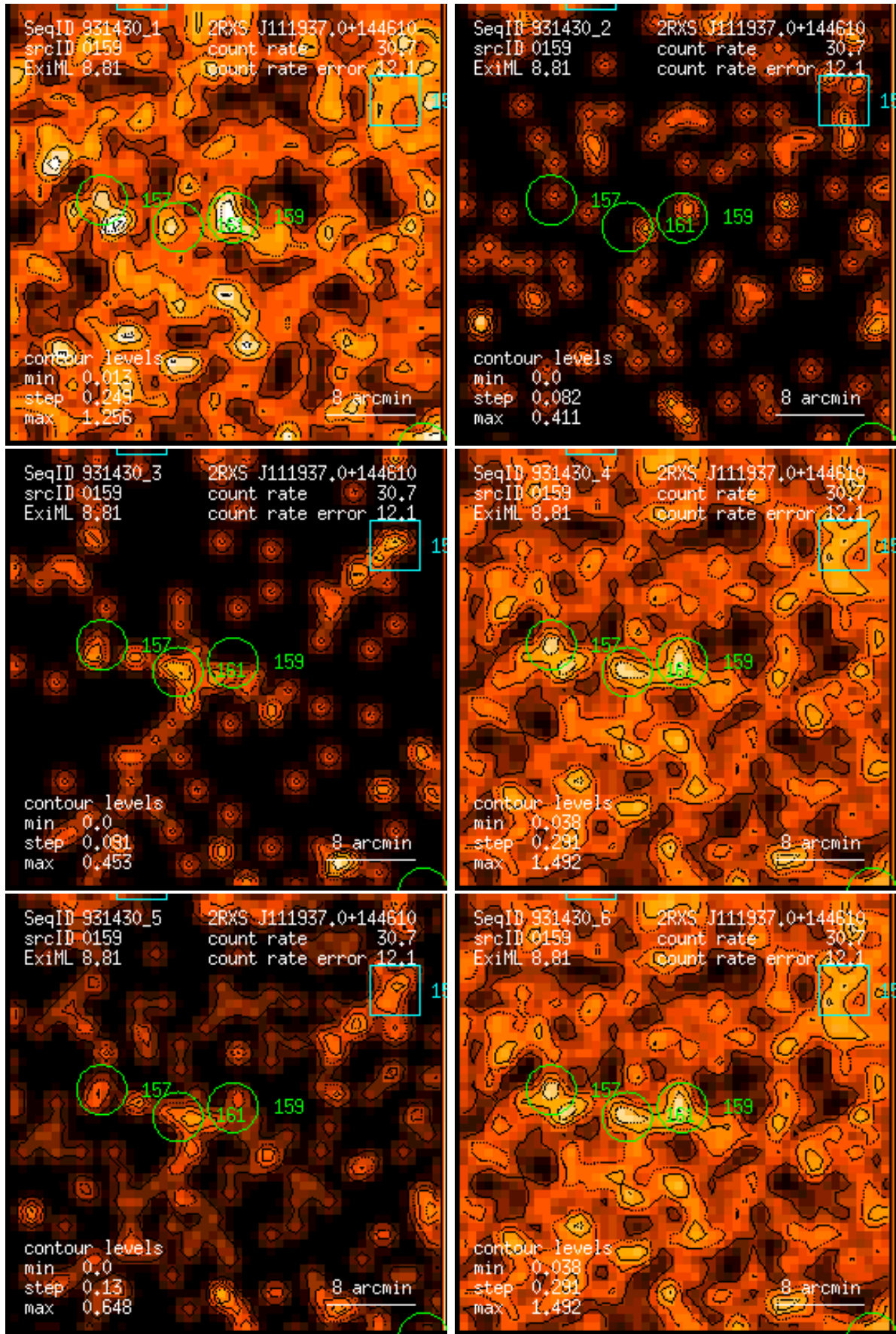
Figure 159: RASS 931430: detection 0159: band rate images, Gaussian filter: (1) PSPC channels 11 – 41, (2) 52 – 90, (3) 91 – 201, (4) 11 – 235, (5) 52 – 201, (6) 11 – 201. Broad band rates in counts/ks. Band rate contour levels in counts/ks/arcmin 2 .
