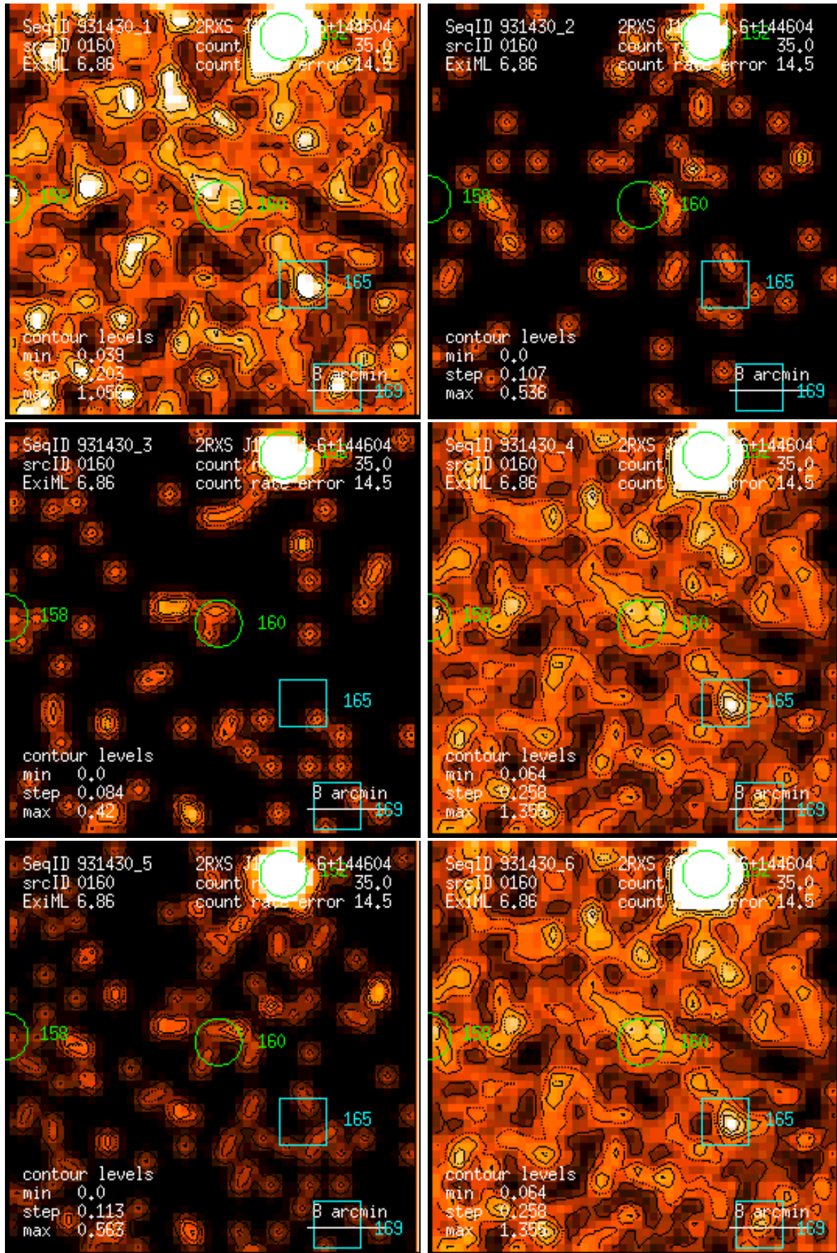
Figure 160: RASS 931430: detection 0160: band rate images, Gaussian filter: (1) PSPC channels 11 – 41, (2) 52 – 90, (3) 91 – 201, (4) 11 – 235, (5) 52 – 201, (6) 11 – 201. Broad band rates in counts/ks. Band rate contour levels in counts/ks/arcmin 2 .
