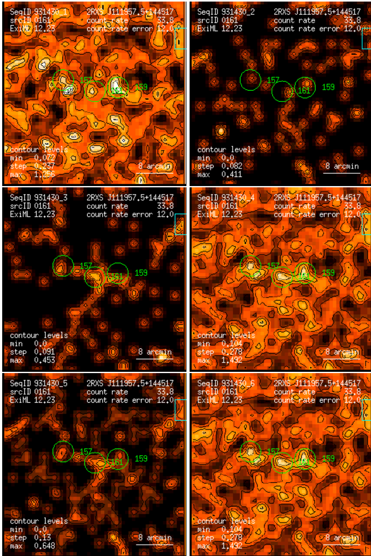
Figure 161: RASS 931430: detection 0161: band rate images, Gaussian filter: (1) PSPC channels 11 – 41, (2) 52 – 90, (3) 91 – 201, (4) 11 – 235, (5) 52 – 201, (6) 11 – 201. Broad band rates in counts/ks. Band rate contour levels in counts/ks/arcmin 2 .
