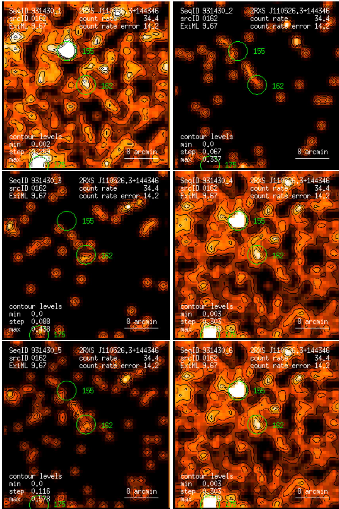
Figure 162: RASS 931430: detection 0162: band rate images, Gaussian filter: (1) PSPC channels 11 – 41, (2) 52 – 90, (3) 91 – 201, (4) 11 – 235, (5) 52 – 201, (6) 11 – 201. Broad band rates in counts/ks. Band rate contour levels in counts/ks/arcmin 2 .
