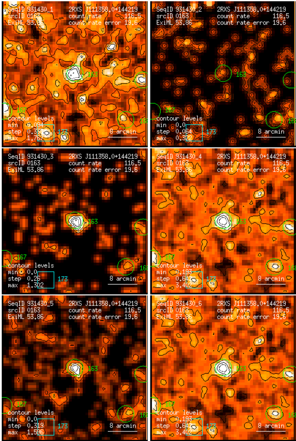
Figure 163: RASS 931430: detection 0163: band rate images, Gaussian filter: (1) PSPC channels 11 – 41, (2) 52 – 90, (3) 91 – 201, (4) 11 – 235, (5) 52 – 201, (6) 11 – 201. Broad band rates in counts/ks. Band rate contour levels in counts/ks/arcmin 2 .
