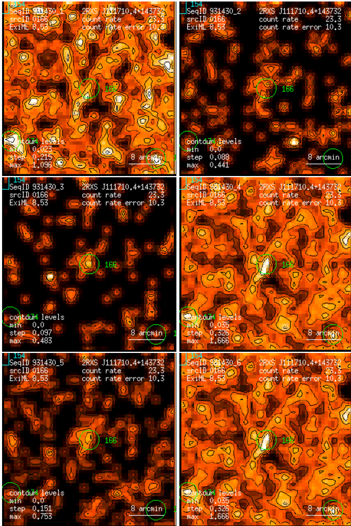
Figure 166: RASS 931430: detection 0166: band rate images, Gaussian filter: (1) PSPC channels 11 – 41, (2) 52 – 90, (3) 91 – 201, (4) 11 – 235, (5) 52 – 201, (6) 11 – 201. Broad band rates in counts/ks. Band rate contour levels in counts/ks/arcmin 2 .
