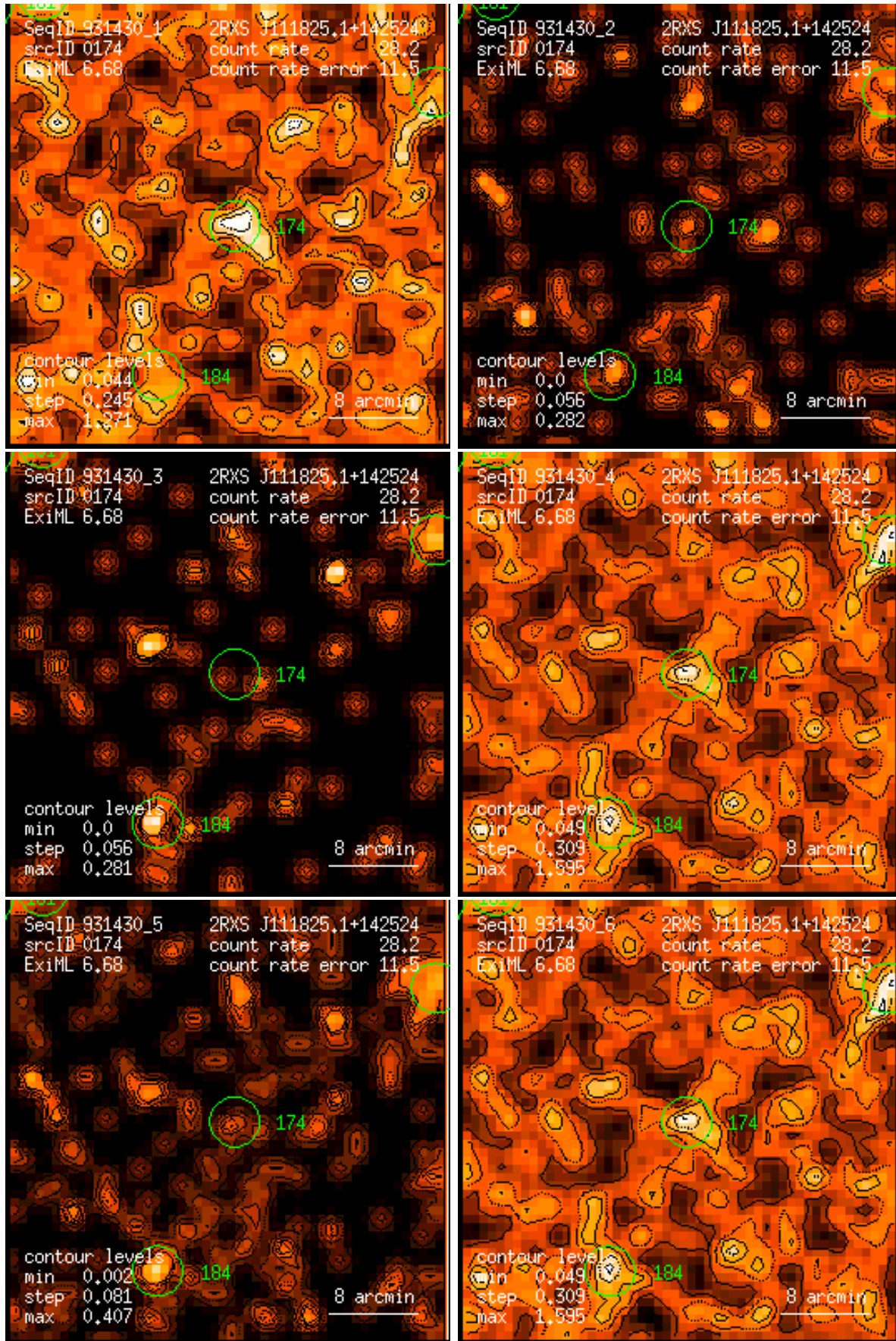
Figure 174: RASS 931430: detection 0174: band rate images, Gaussian filter: (1) PSPC channels 11 – 41, (2) 52 – 90, (3) 91 – 201, (4) 11 – 235, (5) 52 – 201, (6) 11 – 201. Broad band rates in counts/ks. Band rate contour levels in counts/ks/arcmin 2 .
