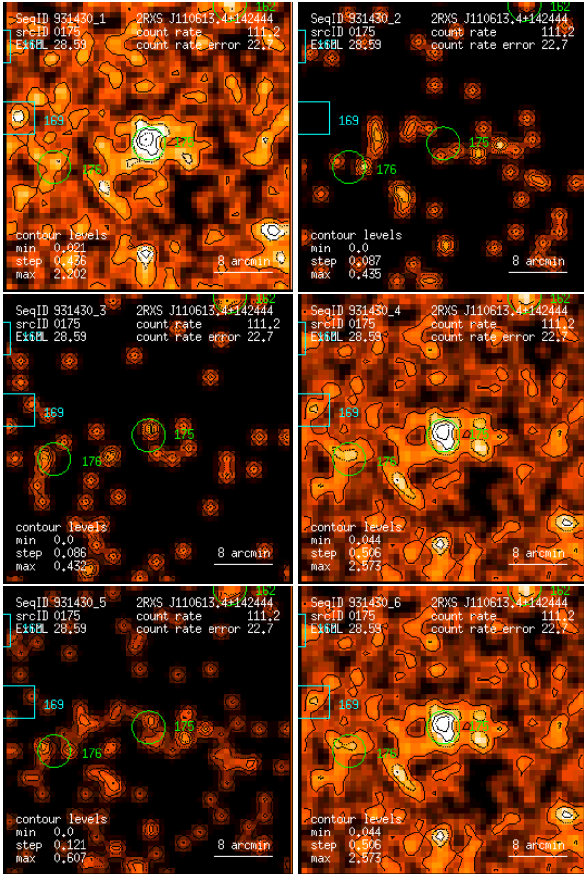
Figure 175: RASS 931430: detection 0175: band rate images, Gaussian filter: (1) PSPC channels 11 – 41, (2) 52 – 90, (3) 91 – 201, (4) 11 – 235, (5) 52 – 201, (6) 11 – 201. Broad band rates in counts/ks. Band rate contour levels in counts/ks/arcmin 2 .
