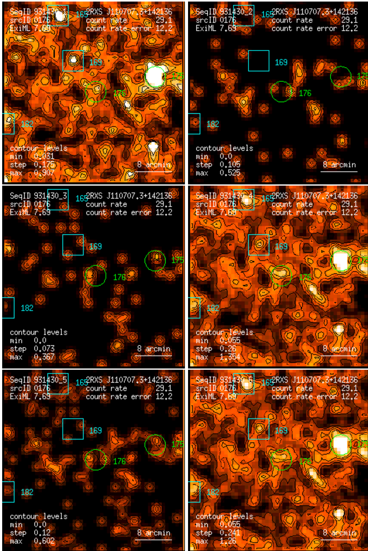
Figure 176: RASS 931430: detection 0176: band rate images, Gaussian filter: (1) PSPC channels 11 – 41, (2) 52 – 90, (3) 91 – 201, (4) 11 – 235, (5) 52 – 201, (6) 11 – 201. Broad band rates in counts/ks. Band rate contour levels in counts/ks/arcmin 2 .
