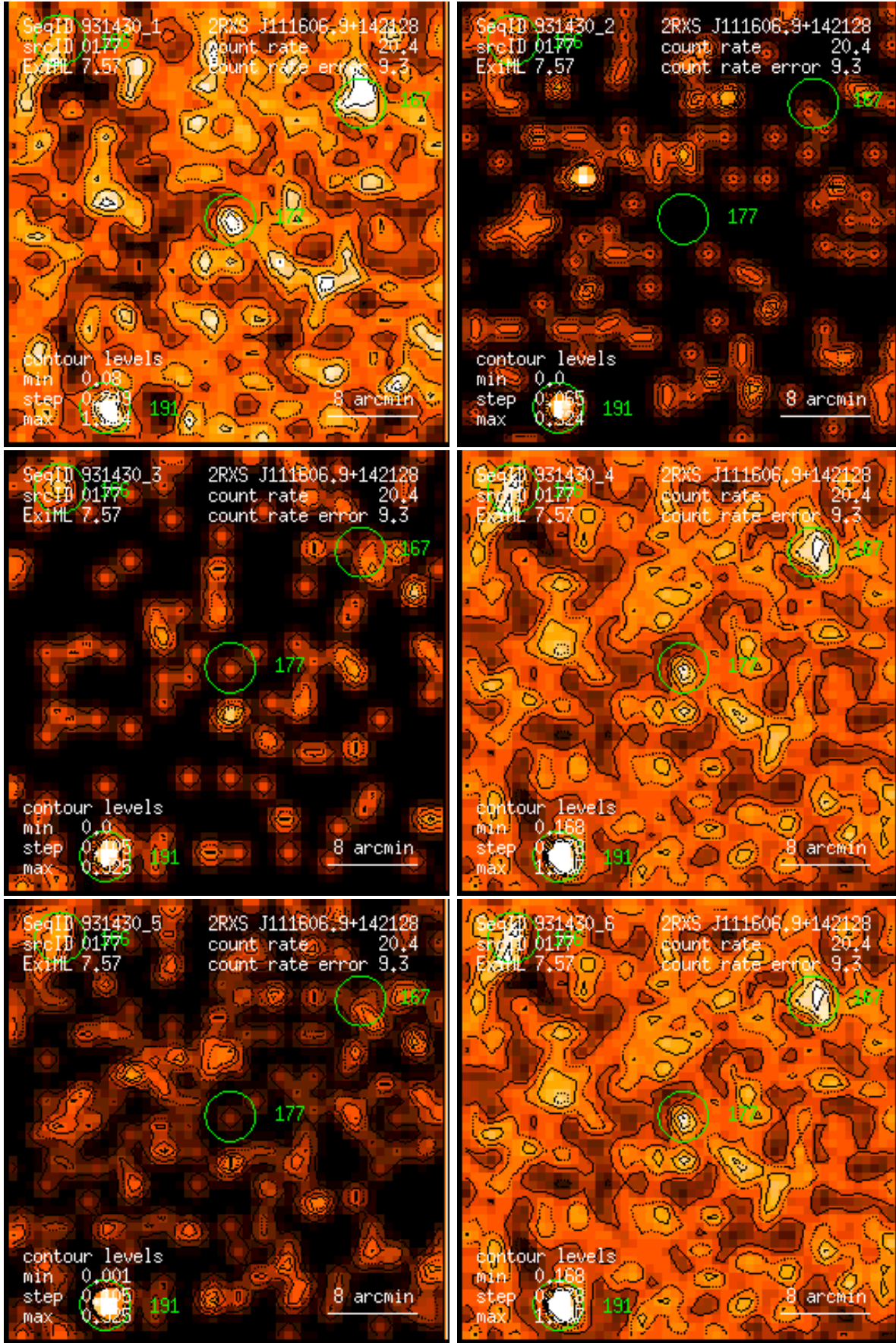
Figure 177: RASS 931430: detection 0177: band rate images, Gaussian filter: (1) PSPC channels 11 – 41, (2) 52 – 90, (3) 91 – 201, (4) 11 – 235, (5) 52 – 201, (6) 11 – 201. Broad band rates in counts/ks. Band rate contour levels in counts/ks/arcmin 2 .
