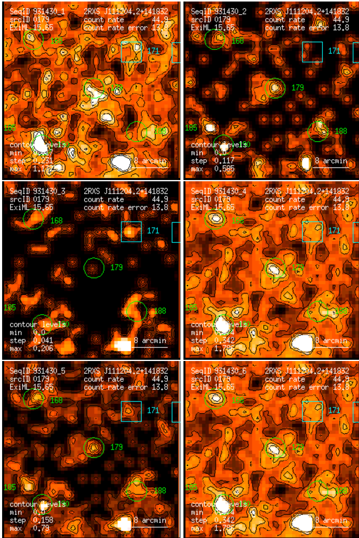
Figure 179: RASS 931430: detection 0179: band rate images, Gaussian filter: (1) PSPC channels 11 – 41, (2) 52 – 90, (3) 91 – 201, (4) 11 – 235, (5) 52 – 201, (6) 11 – 201. Broad band rates in counts/ks. Band rate contour levels in counts/ks/arcmin 2 .
