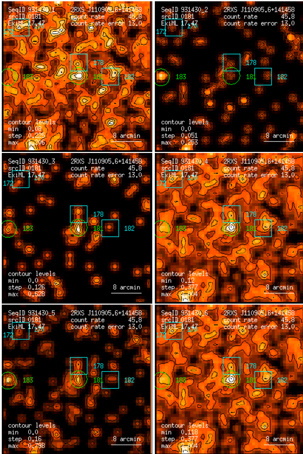
Figure 181: RASS 931430: detection 0181: band rate images, Gaussian filter: (1) PSPC channels 11 – 41, (2) 52 – 90, (3) 91 – 201, (4) 11 – 235, (5) 52 – 201, (6) 11 – 201. Broad band rates in counts/ks. Band rate contour levels in counts/ks/arcmin 2 .
