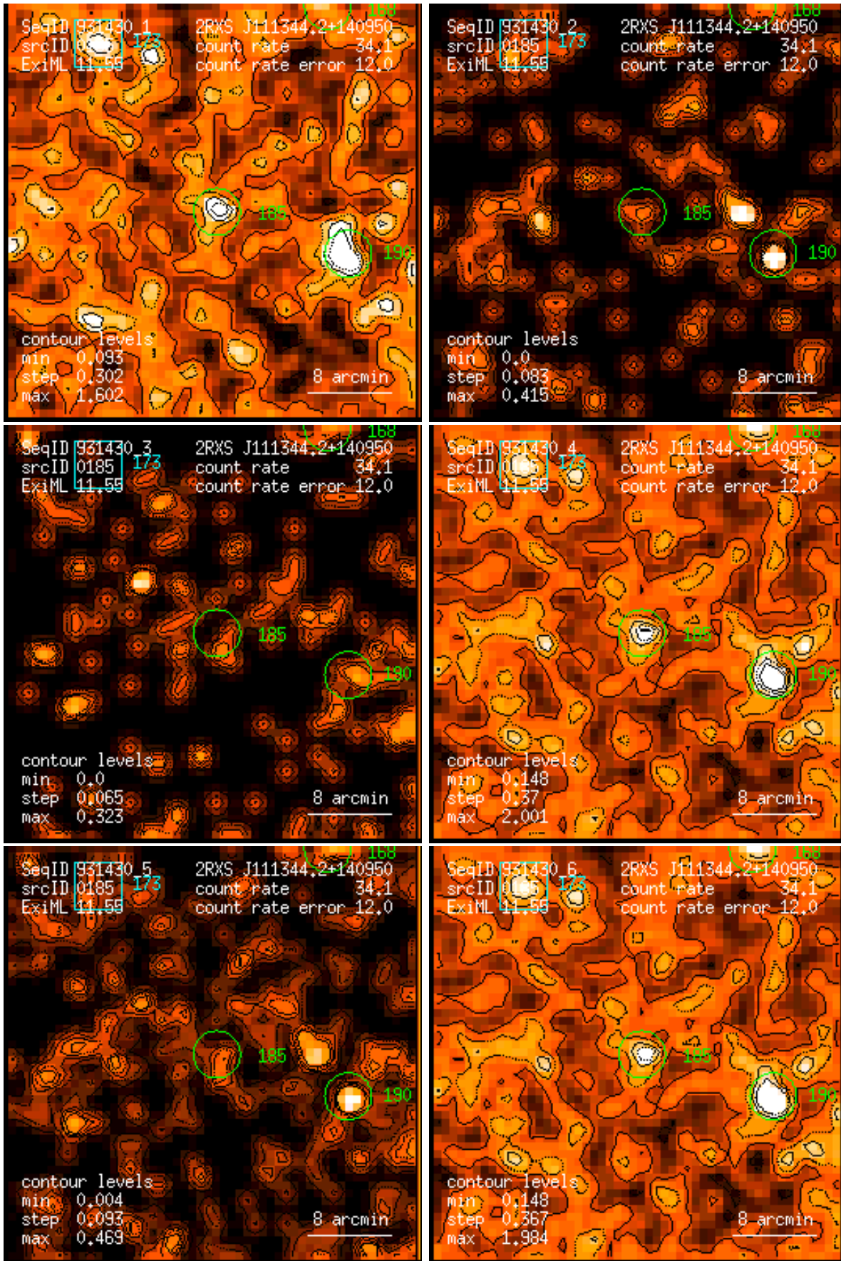
Figure 185: RASS 931430: detection 0185: band rate images, Gaussian filter: (1) PSPC channels 11 – 41, (2) 52 – 90, (3) 91 – 201, (4) 11 – 235, (5) 52 – 201, (6) 11 – 201. Broad band rates in counts/ks. Band rate contour levels in counts/ks/arcmin 2 .
