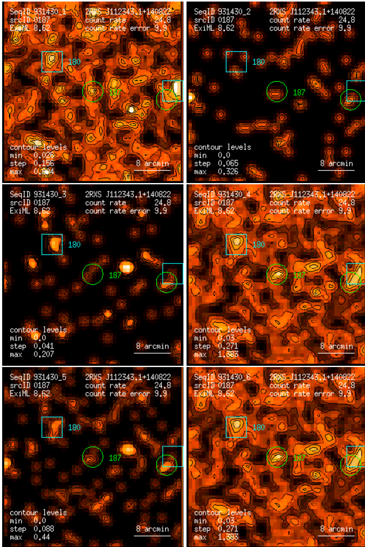
Figure 187: RASS 931430: detection 0187: band rate images, Gaussian filter: (1) PSPC channels 11 – 41, (2) 52 – 90, (3) 91 – 201, (4) 11 – 235, (5) 52 – 201, (6) 11 – 201. Broad band rates in counts/ks. Band rate contour levels in counts/ks/arcmin 2 .
