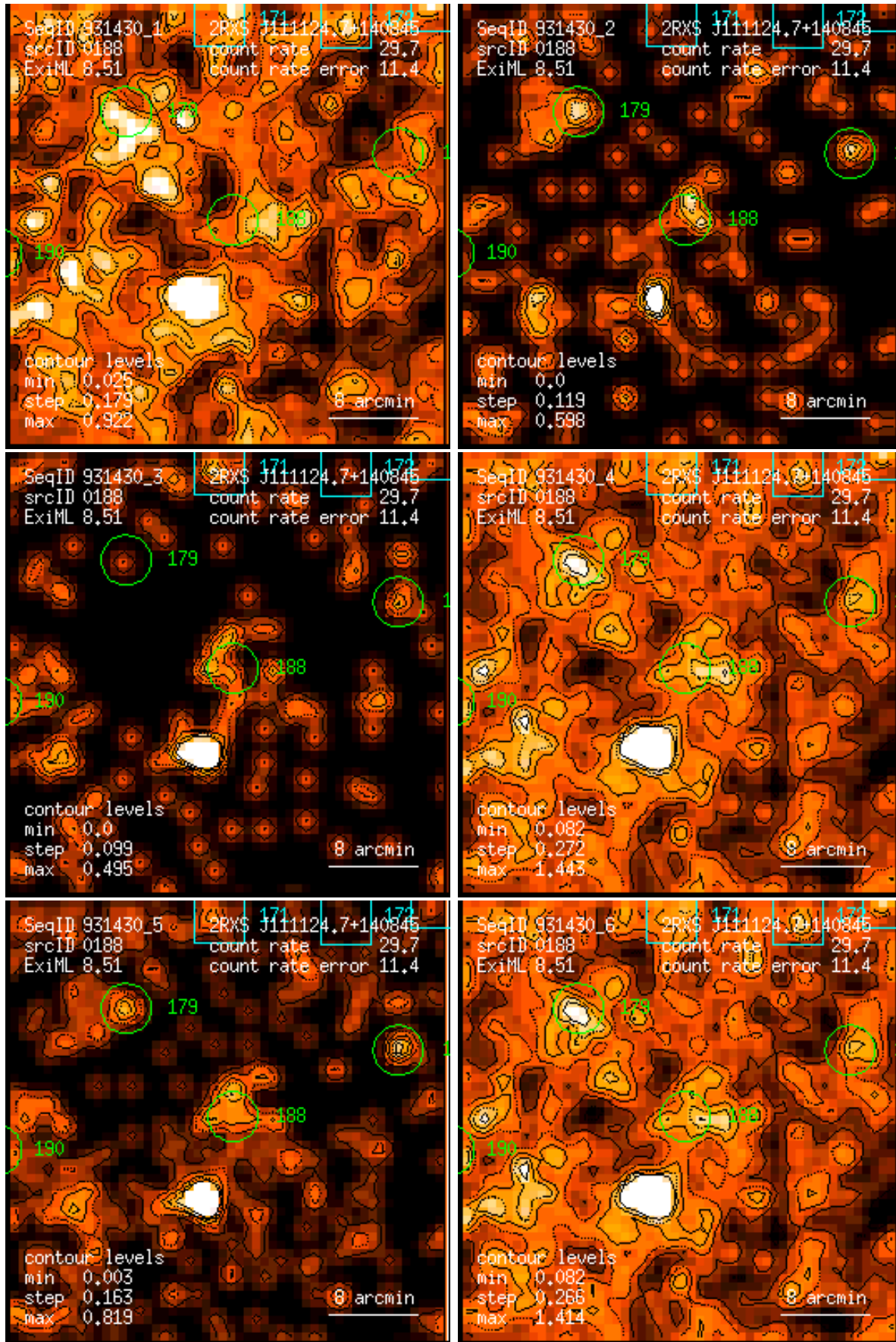
Figure 188: RASS 931430: detection 0188: band rate images, Gaussian filter: (1) PSPC channels 11 – 41, (2) 52 – 90, (3) 91 – 201, (4) 11 – 235, (5) 52 – 201, (6) 11 – 201. Broad band rates in counts/ks. Band rate contour levels in counts/ks/arcmin 2 .
