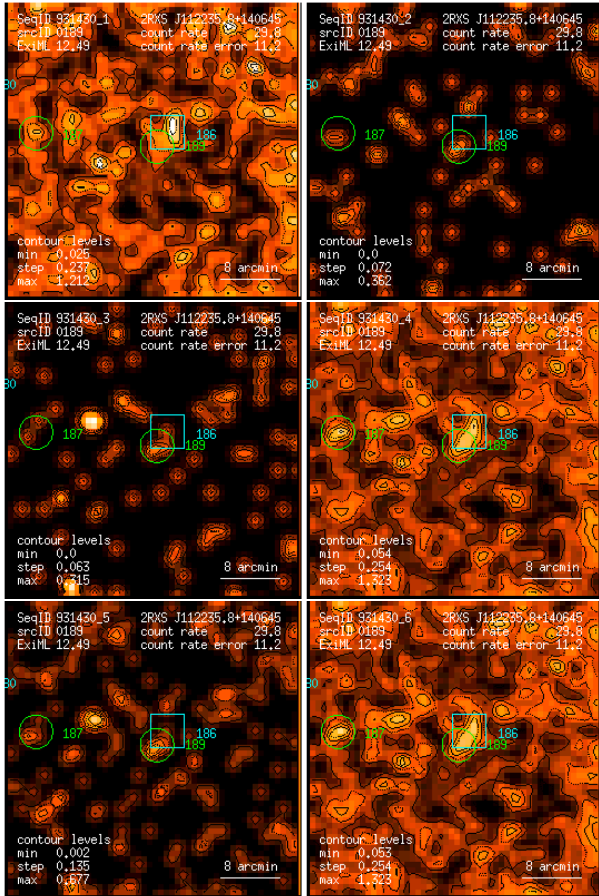
Figure 189: RASS 931430: detection 0189: band rate images, Gaussian filter: (1) PSPC channels 11 – 41, (2) 52 – 90, (3) 91 – 201, (4) 11 – 235, (5) 52 – 201, (6) 11 – 201. Broad band rates in counts/ks. Band rate contour levels in counts/ks/arcmin 2 .
