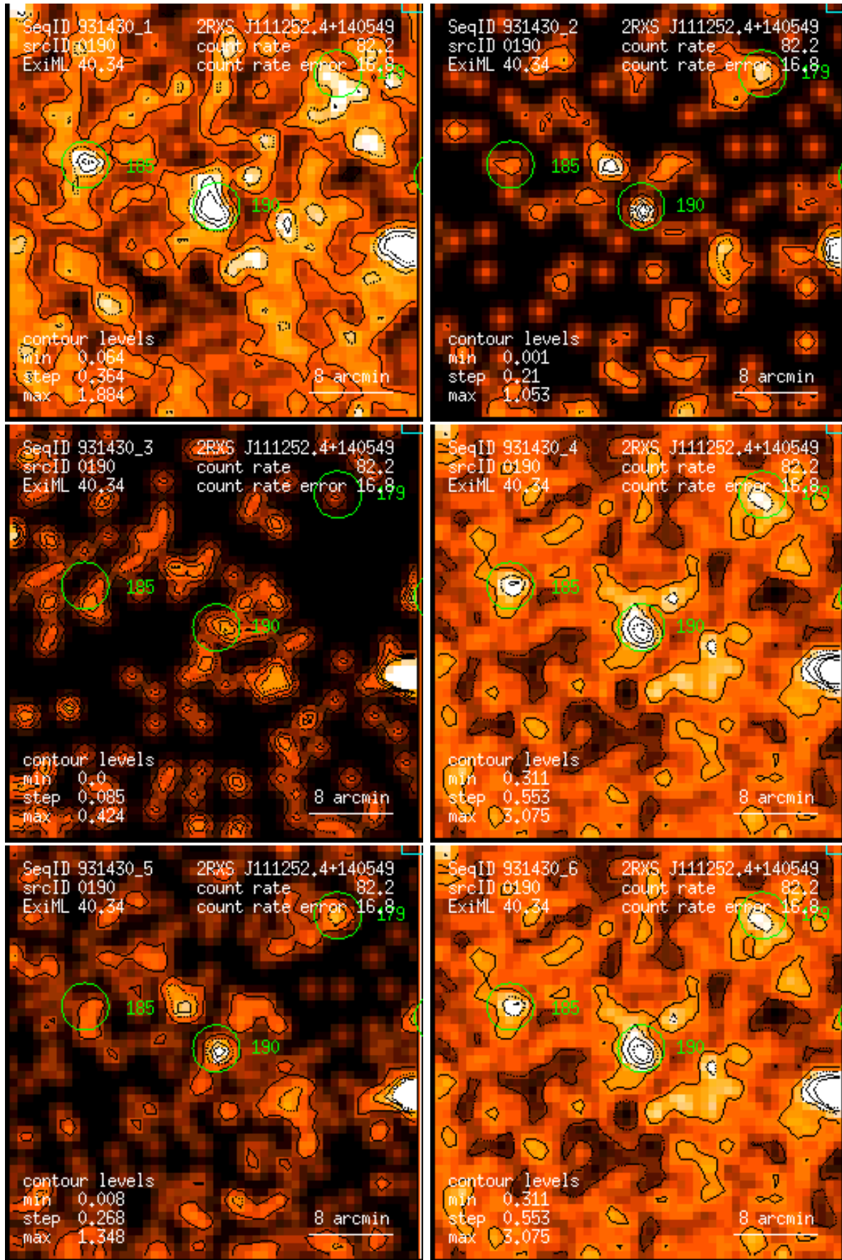
Figure 190: RASS 931430: detection 0190: band rate images, Gaussian filter: (1) PSPC channels 11 – 41, (2) 52 – 90, (3) 91 – 201, (4) 11 – 235, (5) 52 – 201, (6) 11 – 201. Broad band rates in counts/ks. Band rate contour levels in counts/ks/arcmin 2 .
