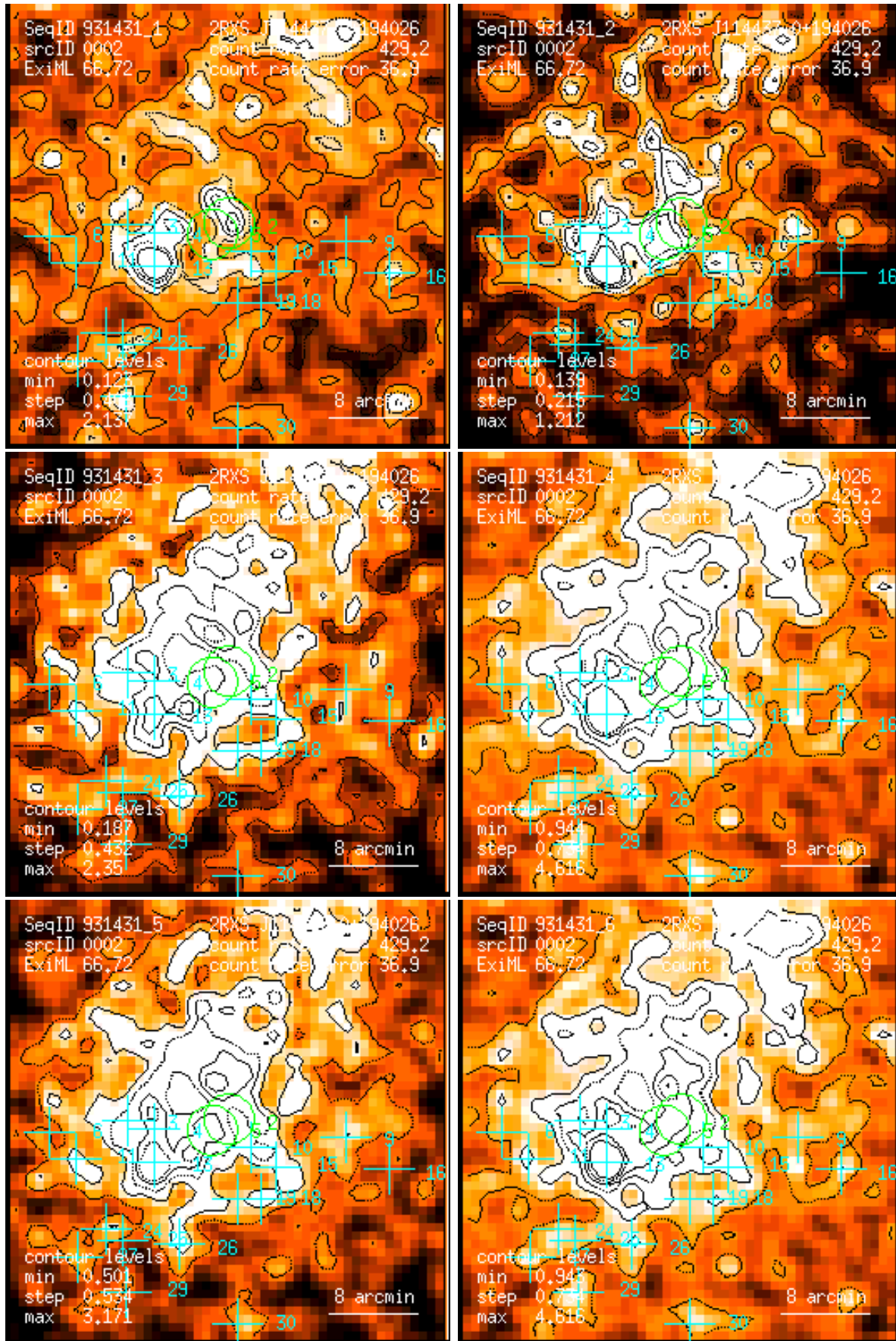
Figure 2: RASS 931431: detection 0002: band rate images, Gaussian filter: (1) PSPC channels 11 – 41, (2) 52 – 90, (3) 91 – 201, (4) 11 – 235, (5) 52 – 201, (6) 11 – 201. Broad band rates in counts/ks. Band rate contour levels in counts/ks/arcmin 2 .
