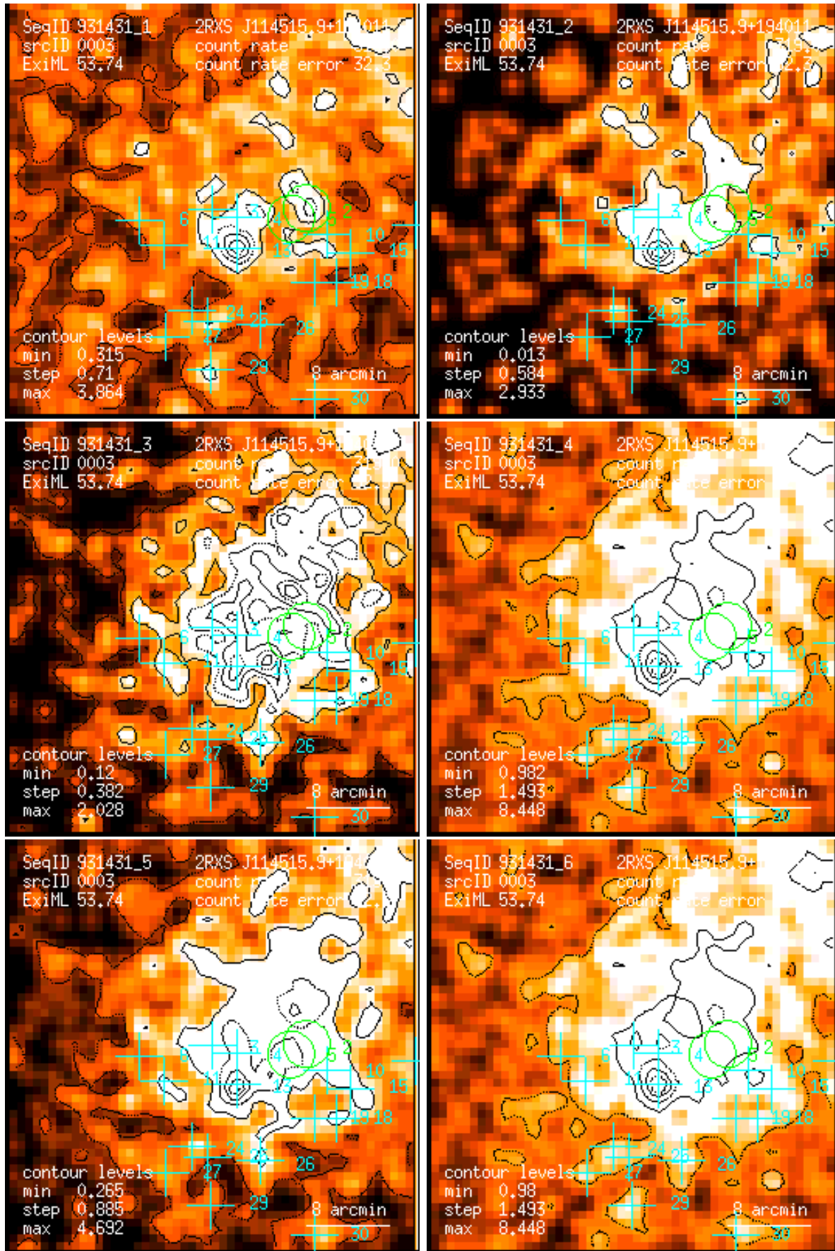
Figure 3: RASS 931431: detection 0003: band rate images, Gaussian filter: (1) PSPC channels 11 – 41, (2) 52 – 90, (3) 91 – 201, (4) 11 – 235, (5) 52 – 201, (6) 11 – 201. Broad band rates in counts/ks. Band rate contour levels in counts/ks/arcmin 2 .
