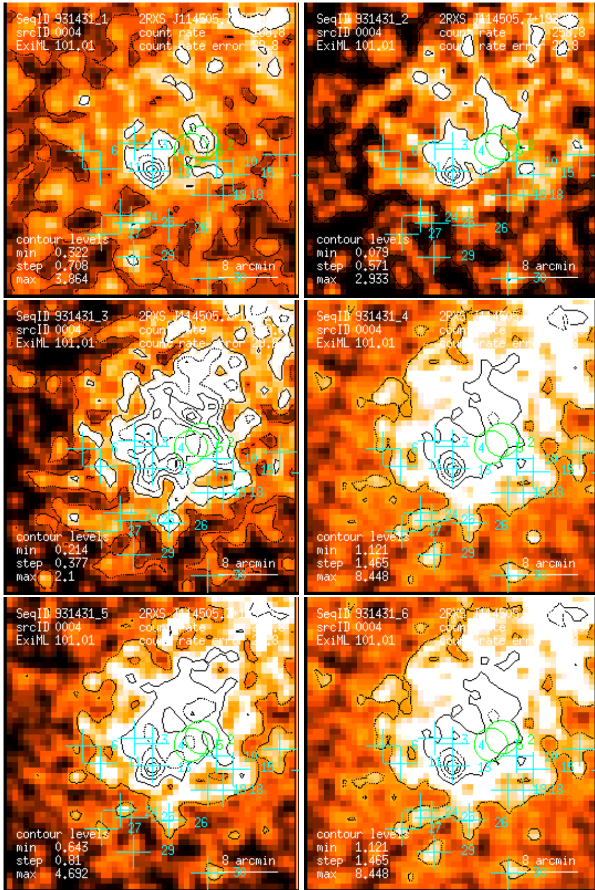
Figure 4: RASS 931431: detection 0004: band rate images, Gaussian filter: (1) PSPC channels 11 – 41, (2) 52 – 90, (3) 91 – 201, (4) 11 – 235, (5) 52 – 201, (6) 11 – 201. Broad band rates in counts/ks. Band rate contour levels in counts/ks/arcmin 2 .
